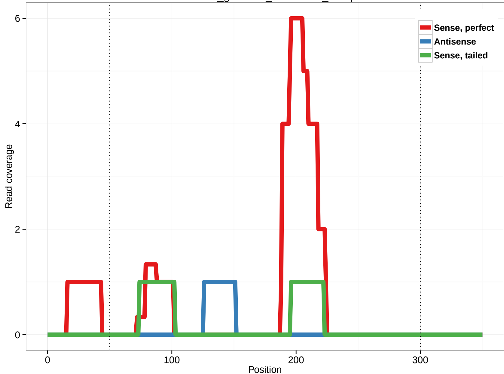
rheMac3_genscan_chr1.2209_25.3p
