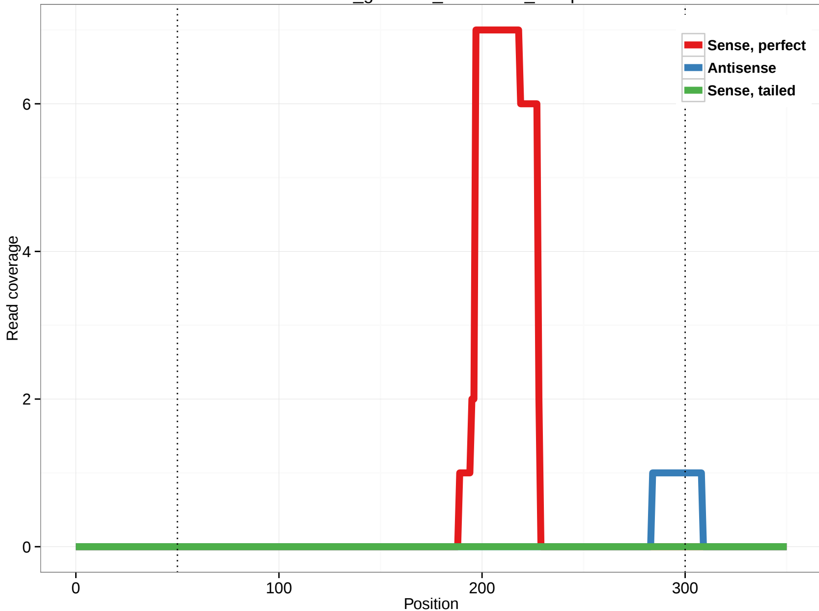
rheMac3_genscan_chr1.2202_10.3p
