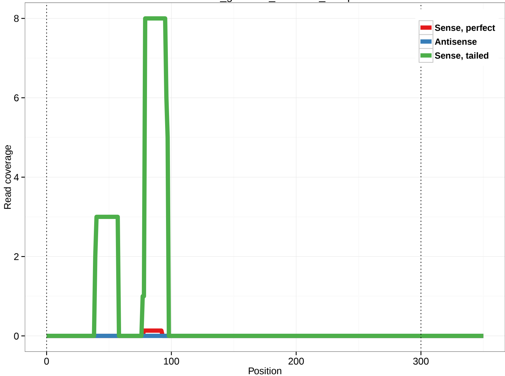
rheMac3_genscan_chr1.215_10.3p
