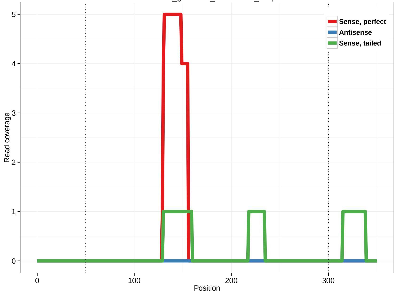
rheMac3_genscan_chr1.2154_4.5p
