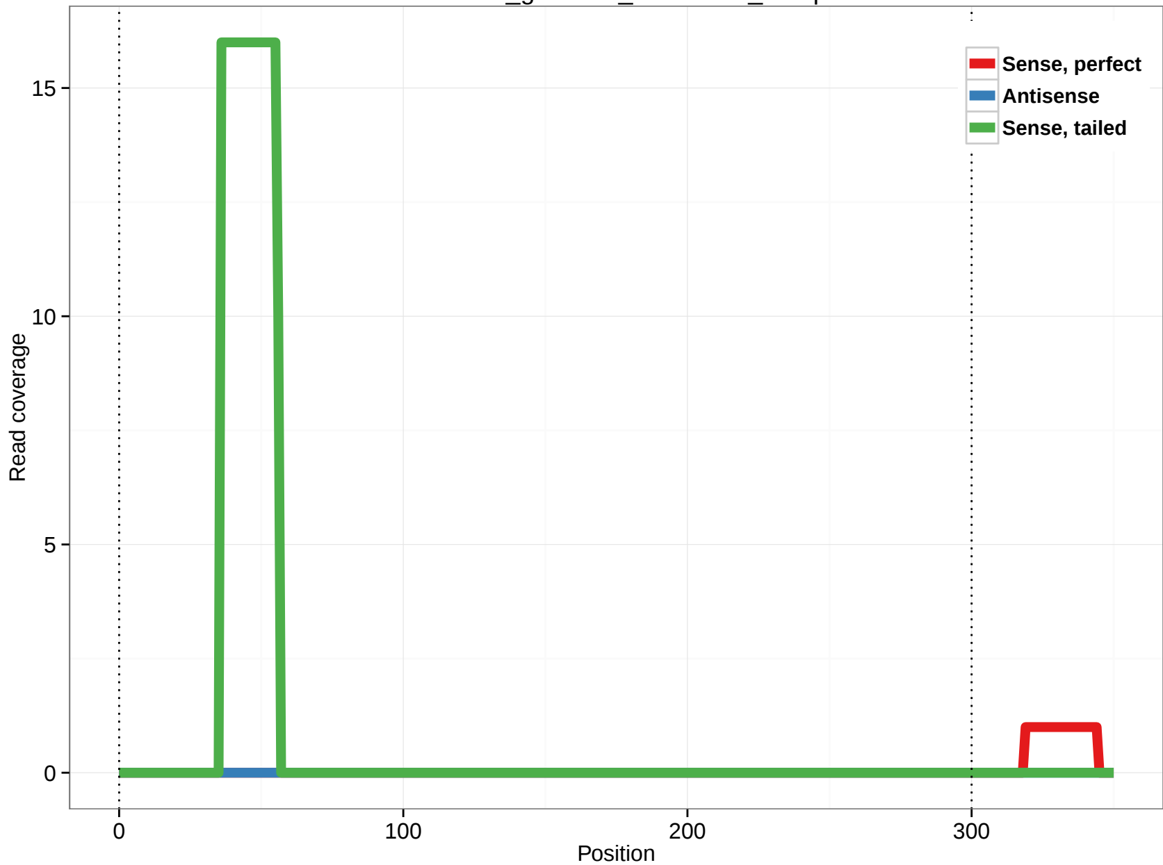
rheMac3_genscan_chr1.2091_26.3p
