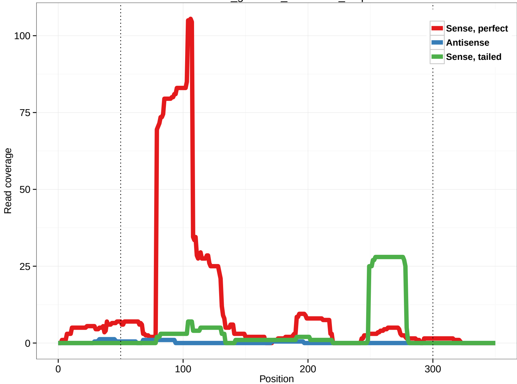
rheMac3_genscan_chr1.1981_3.5p
