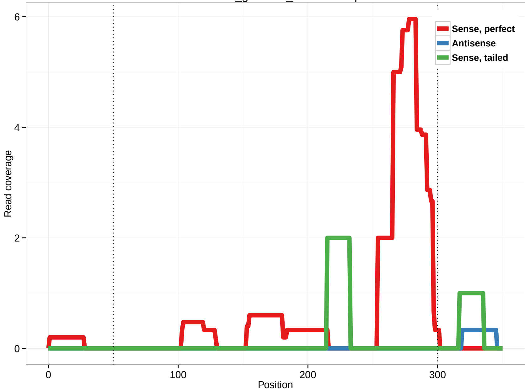
rheMac3_genscan_chr1.1970.5p
