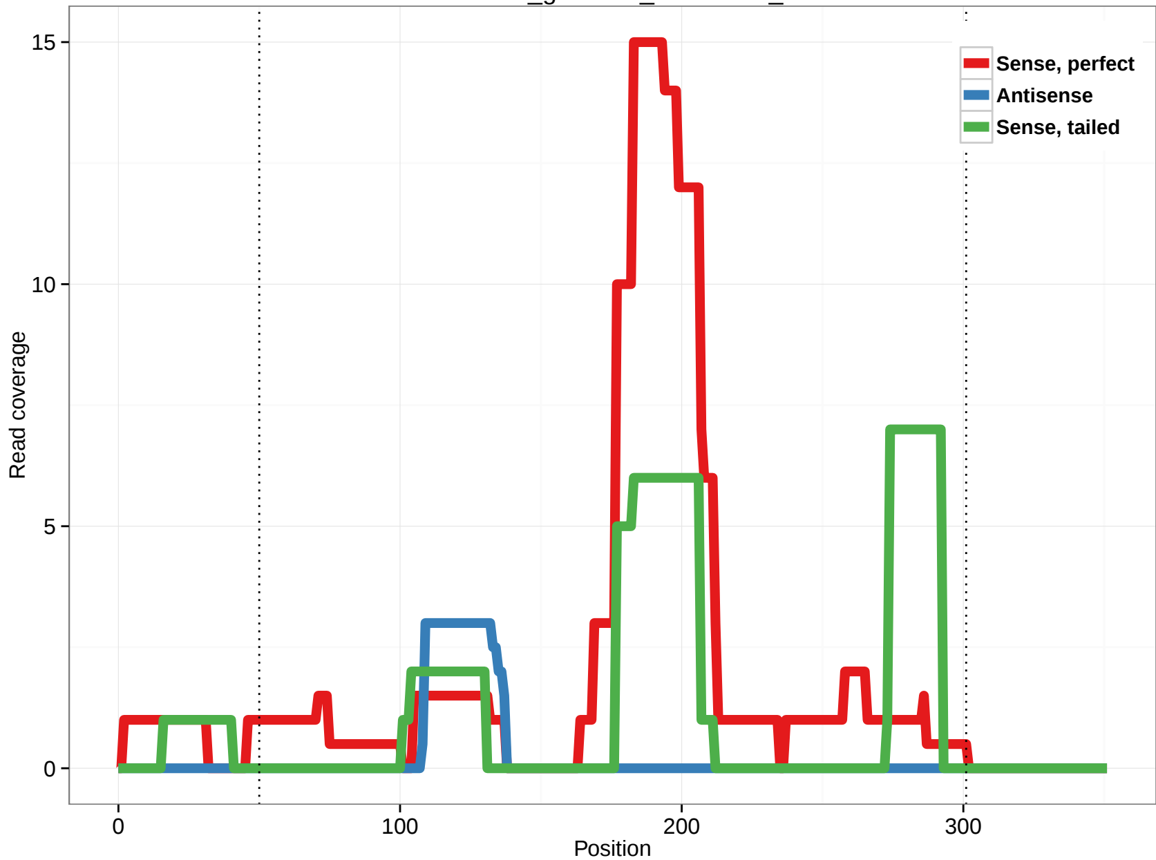
rheMac3_genscan_chr1.1962_1
