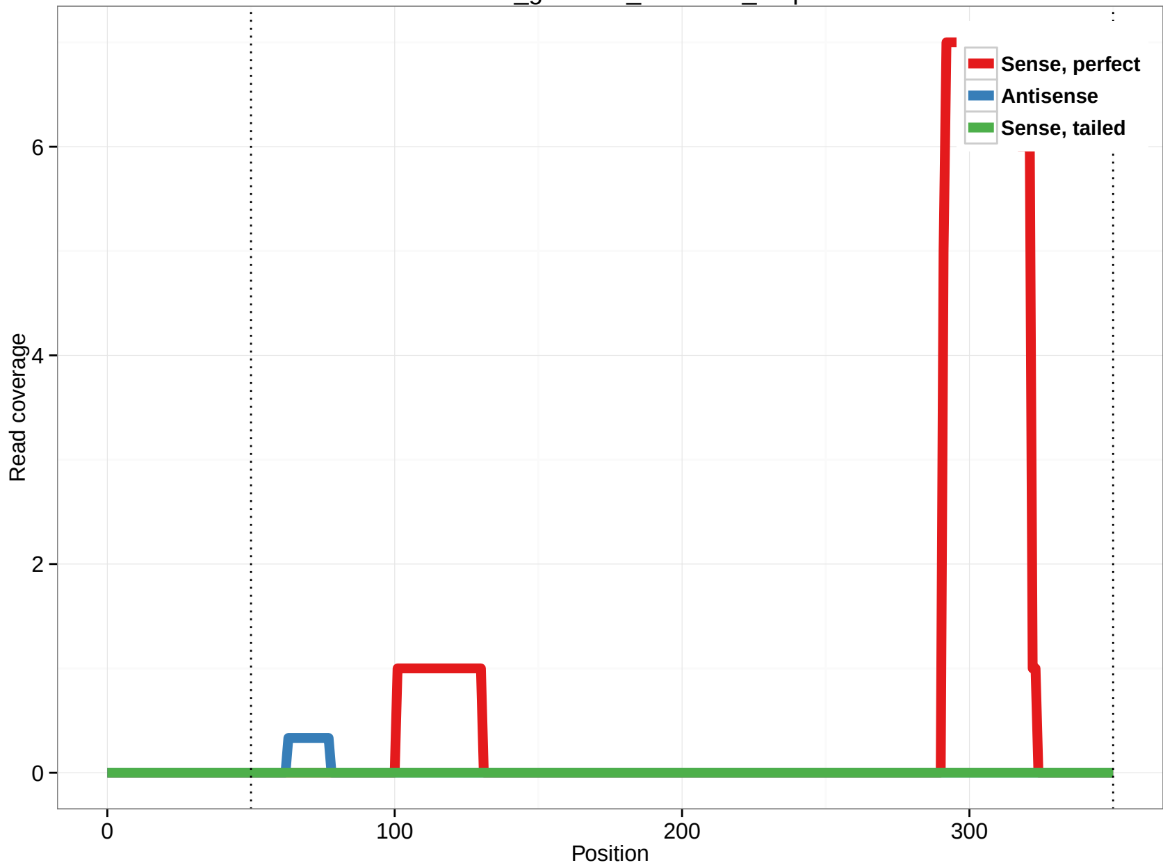
rheMac3_genscan_chr1.191_8.5p
