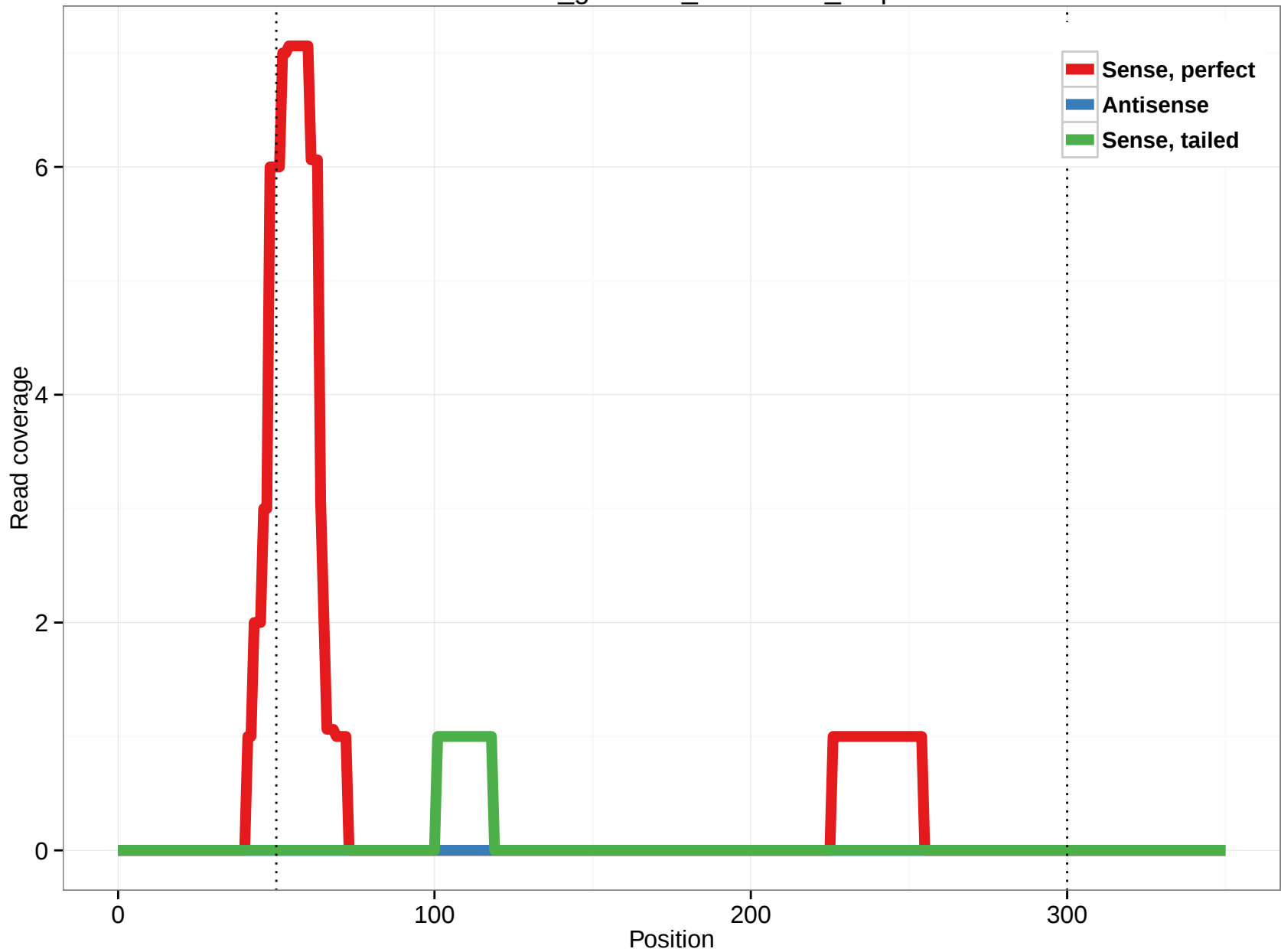
rheMac3_genscan_chr1.1902_0.5p
