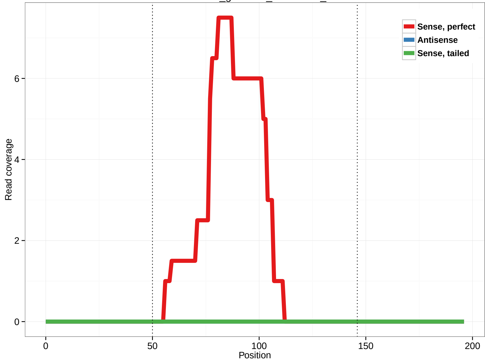
rheMac3_genscan_chr1.1866_0
