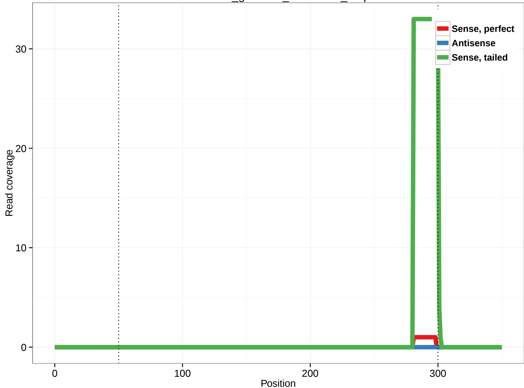
rheMac3_genscan_chr1.1811_1.3p
