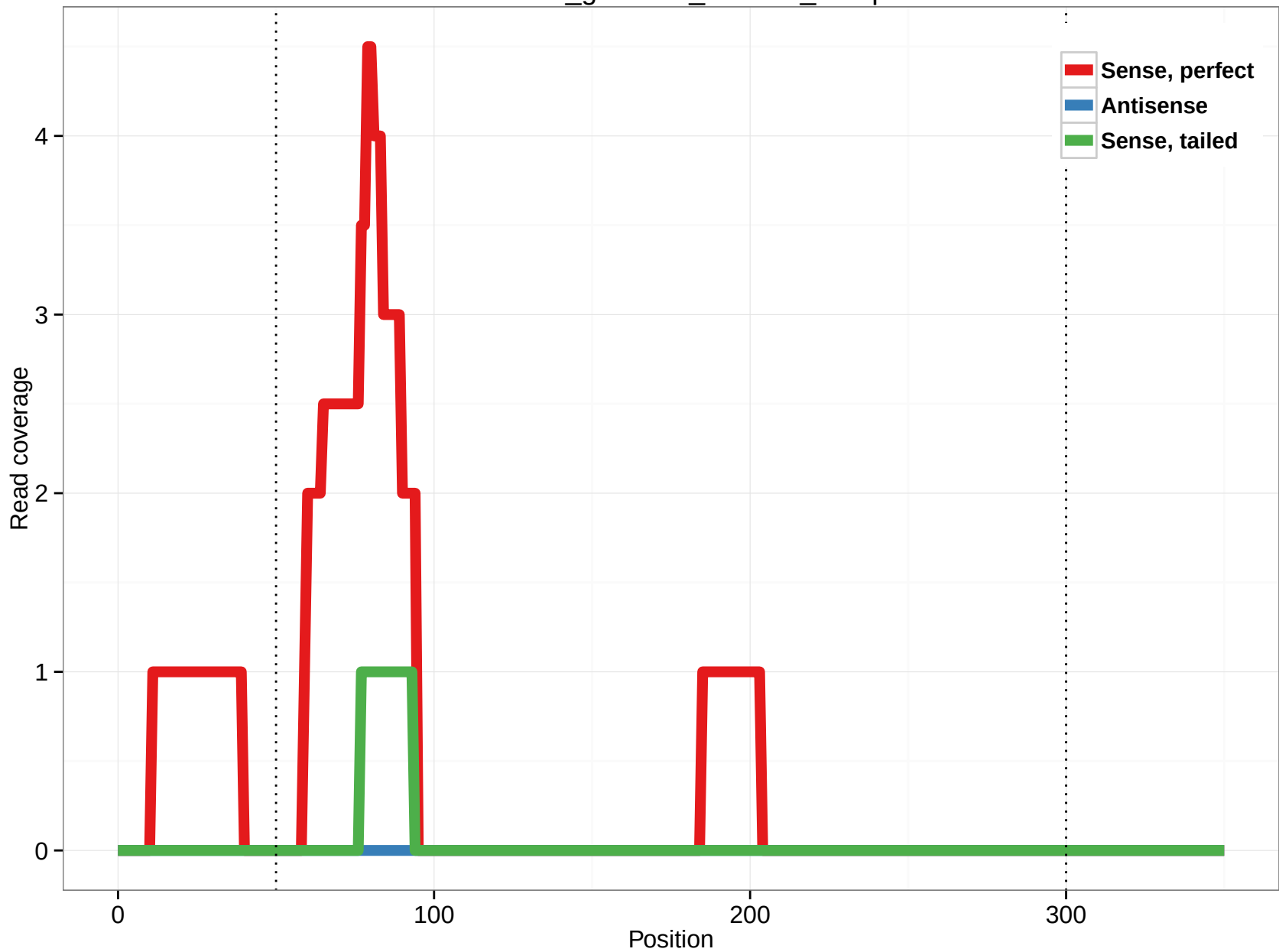
rheMac3_genscan_chr1.17_73.5p
