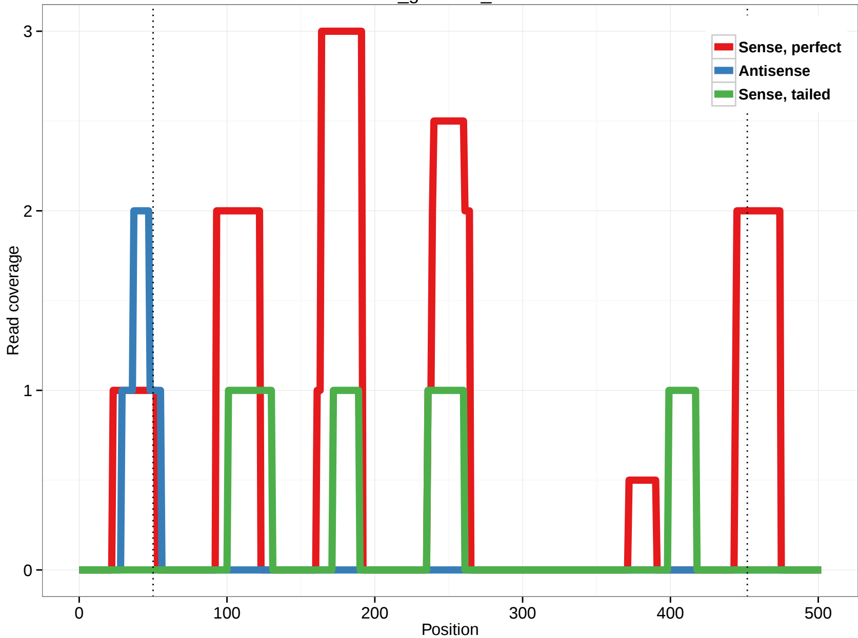
rheMac3_genscan_chr1.1786
