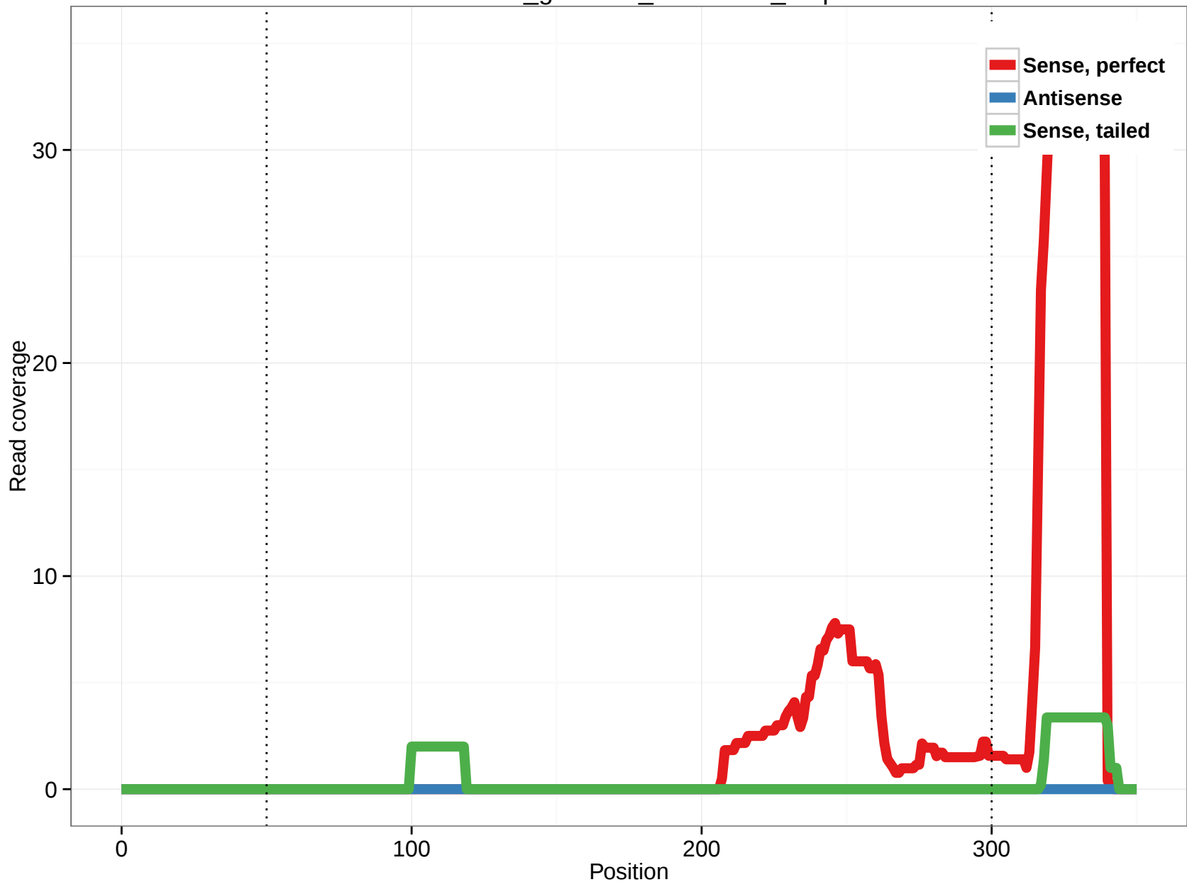
rheMac3_genscan_chr1.1762_1.3p
