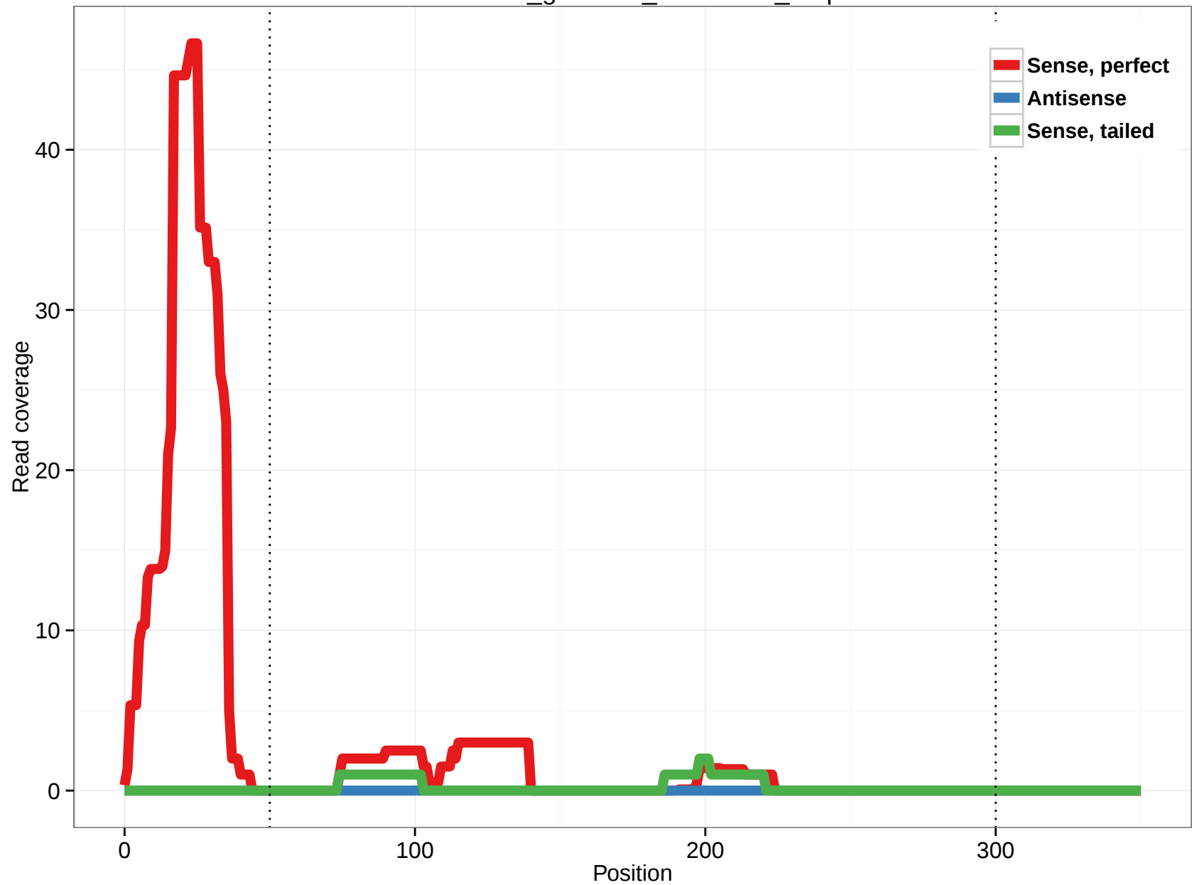
rheMac3_genscan_chr1.1656_0.3p
