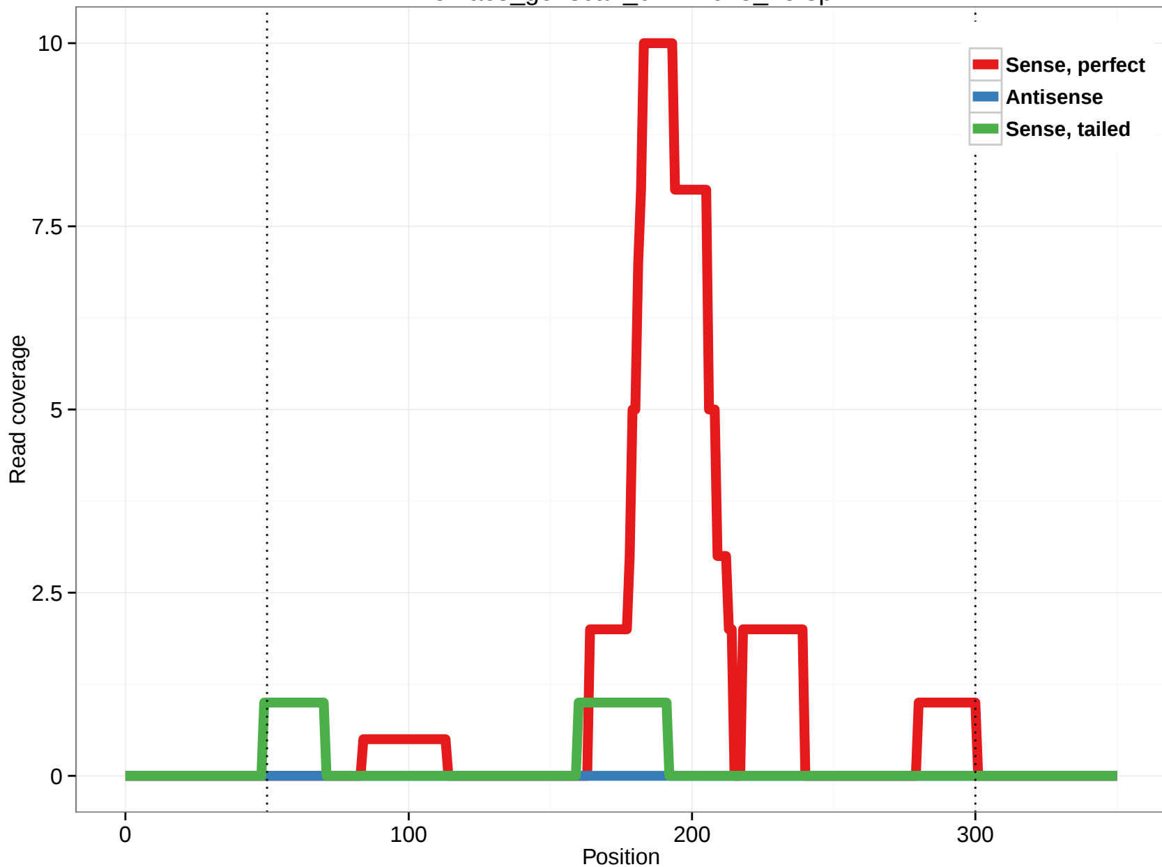
rheMac3_genscan_chr1.1625_13.3p
