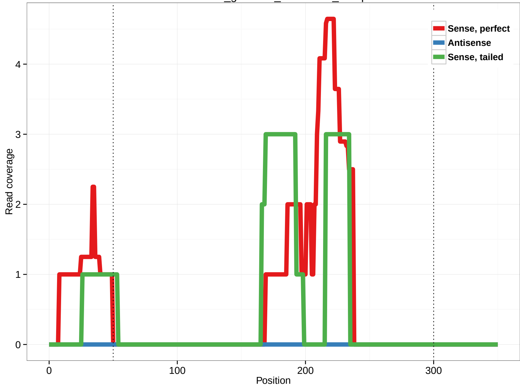
rheMac3_genscan_chr1.1625_10.5p
