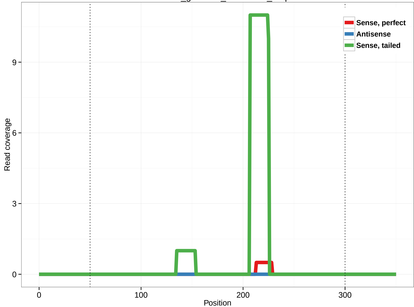
rheMac3_genscan_chr1.1613_2.5p
