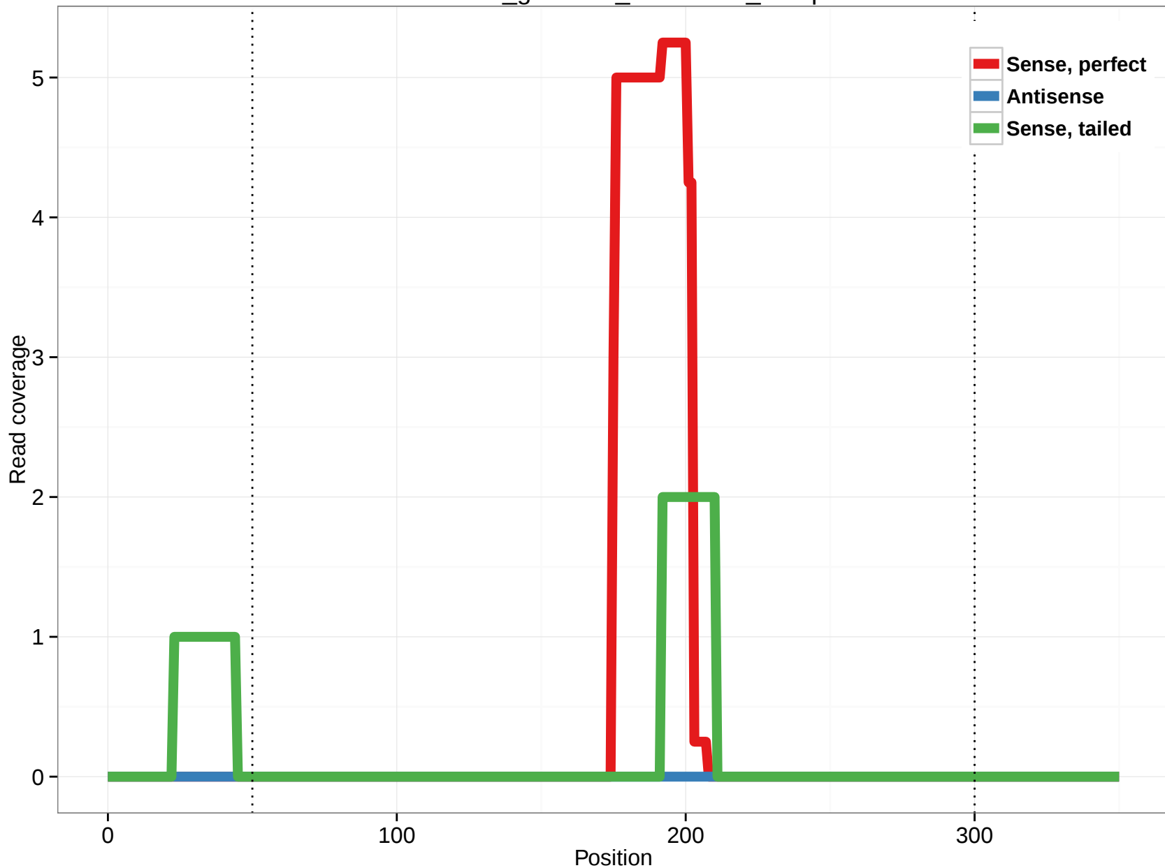
rheMac3_genscan_chr1.1570_24.3p
