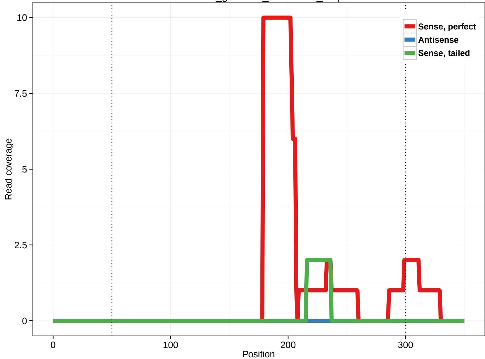
rheMac3_genscan_chr1.1555_1.5p
