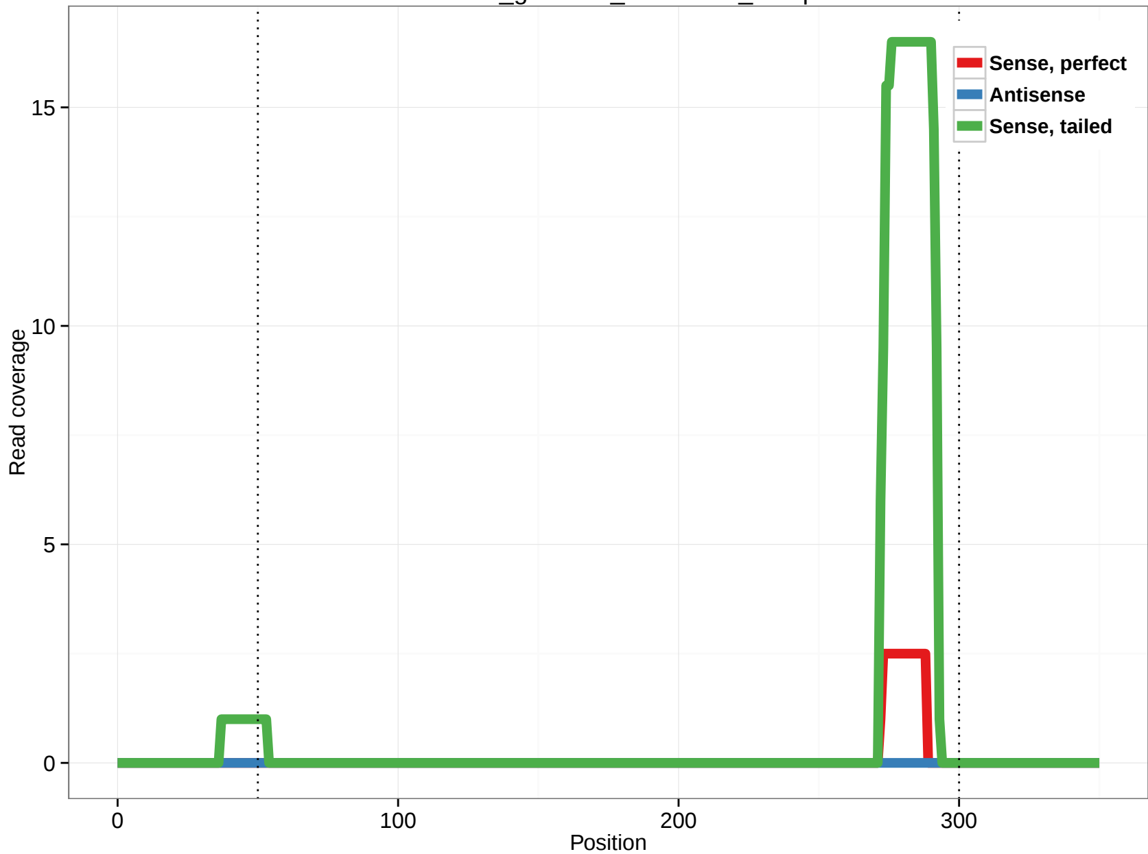
rheMac3_genscan_chr1.1491_15.5p
