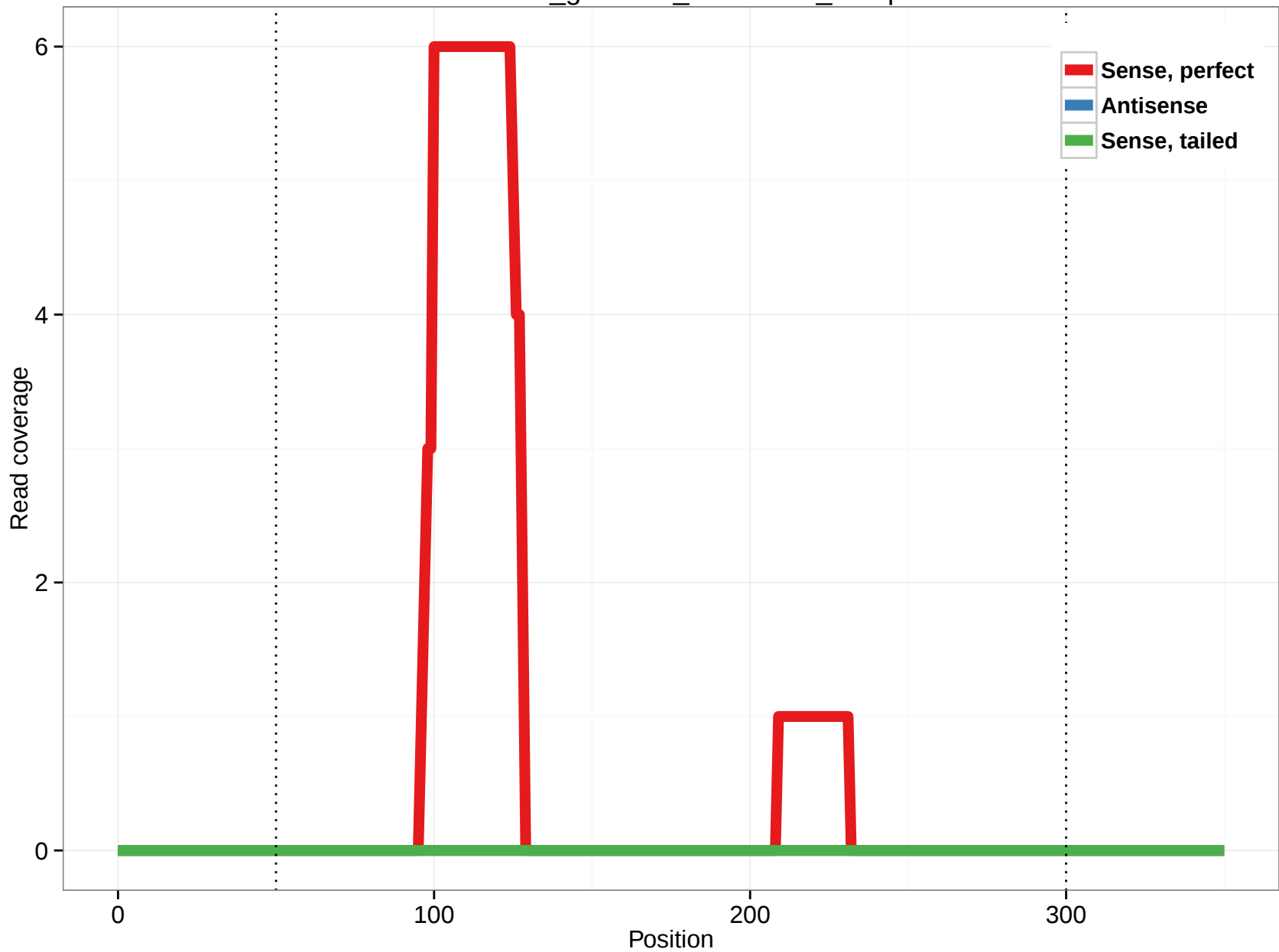
rheMac3_genscan_chr1.1469_18.5p
