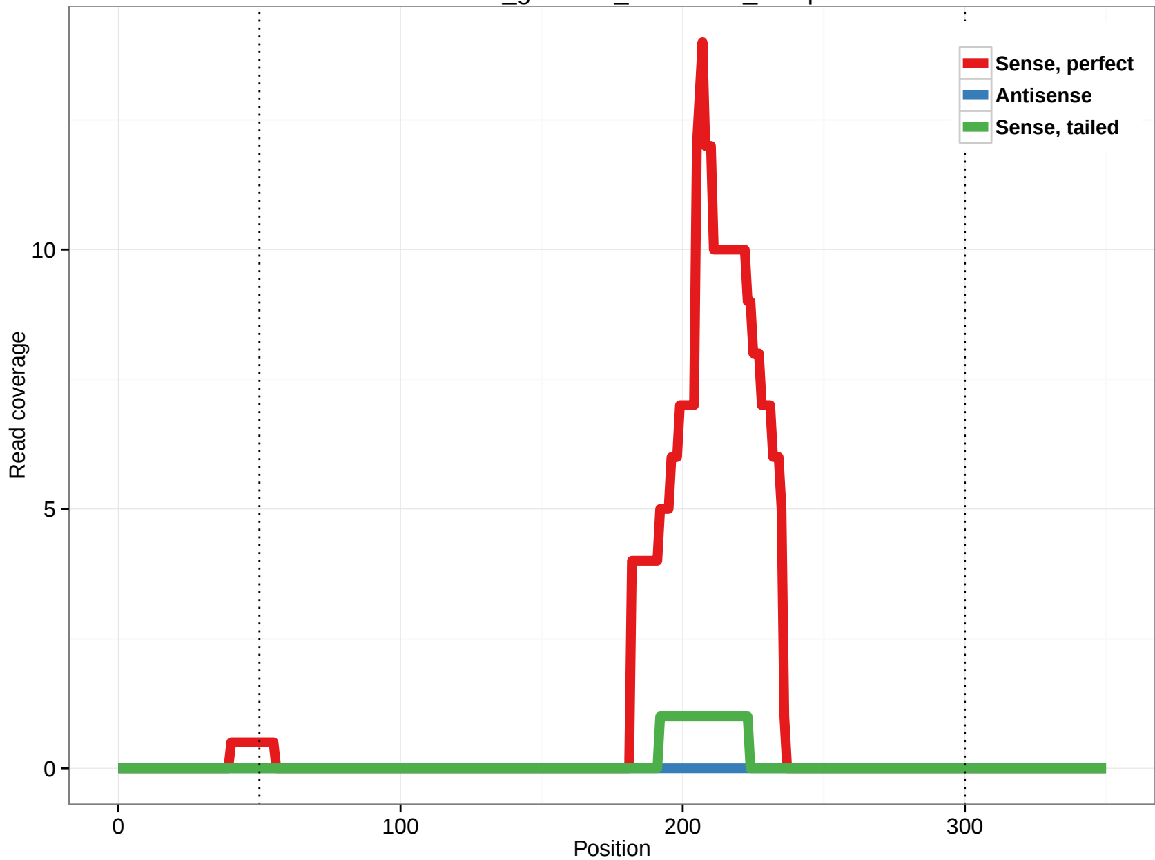
rheMac3_genscan_chr1.1468_10.3p
