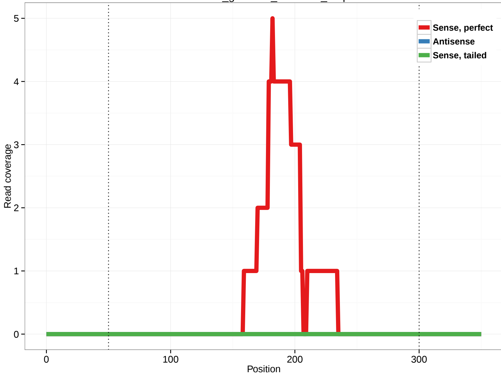
rheMac3_genscan_chr1.144_3.3p
