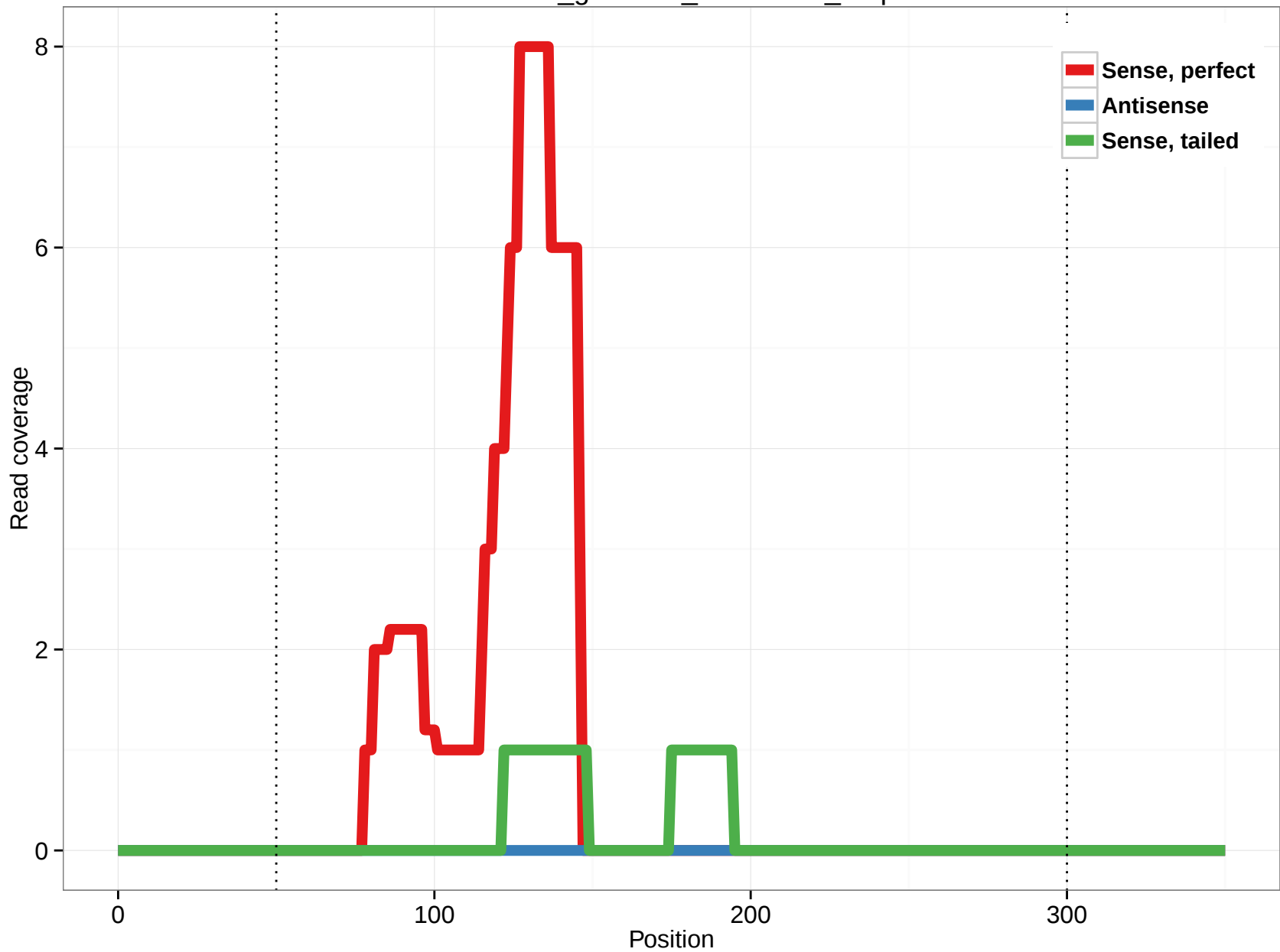
rheMac3_genscan_chr1.1437_6.5p
