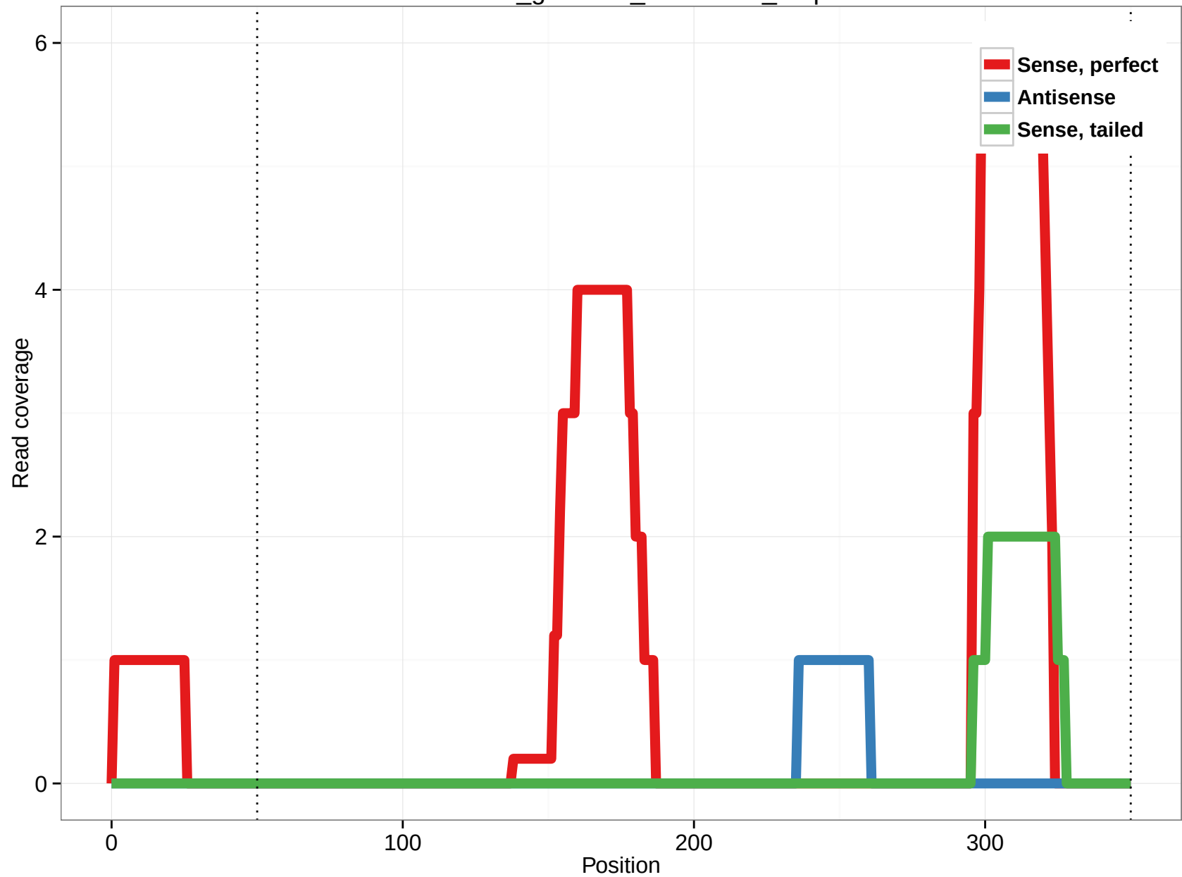
rheMac3_genscan_chr1.1384_5.5p
