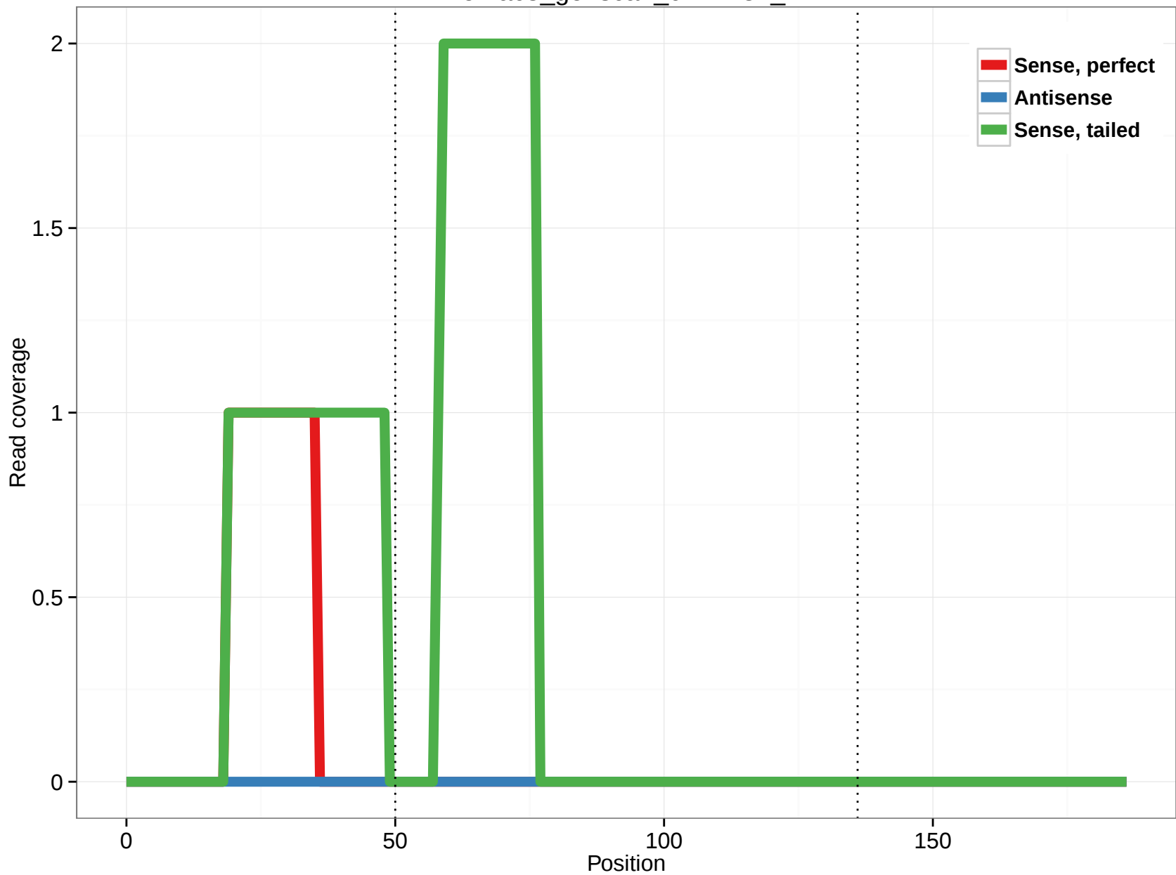
rheMac3_genscan_chr1.137_12
