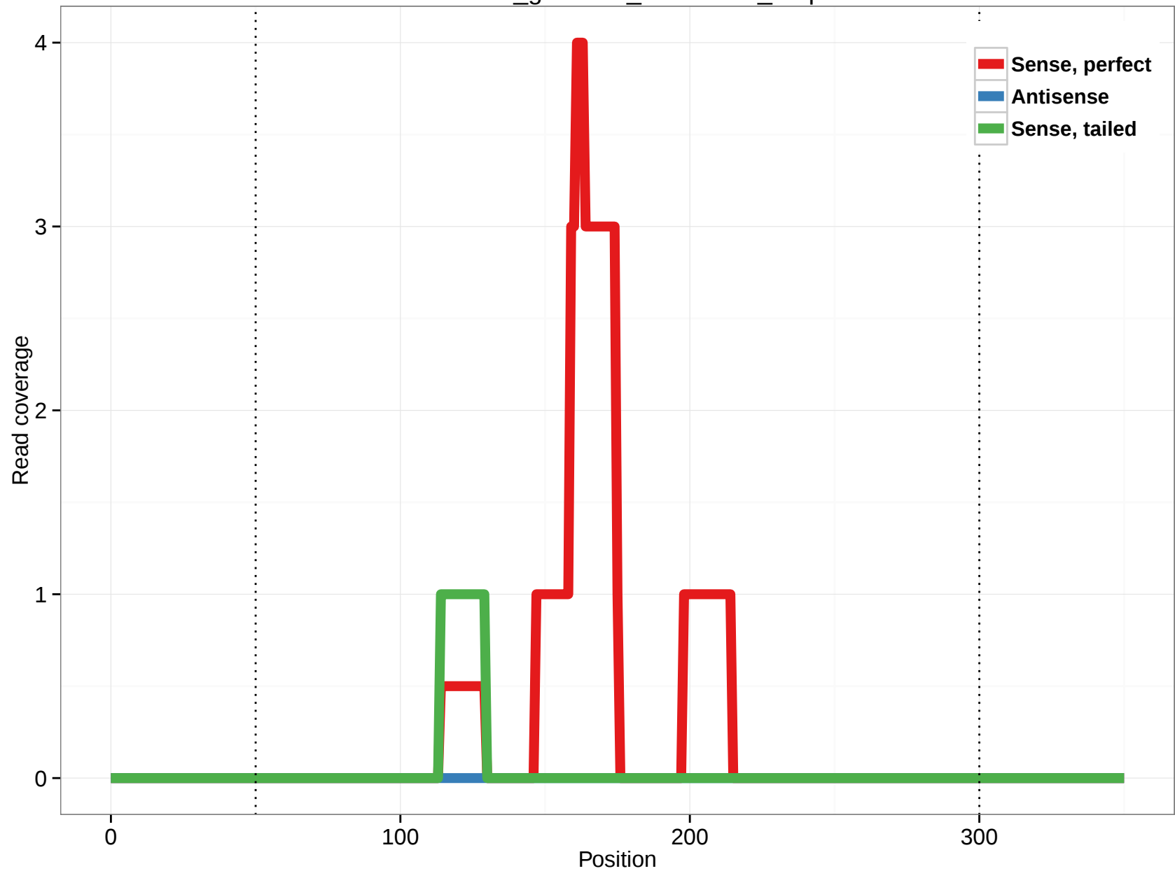
rheMac3_genscan_chr1.1377_1.5p
