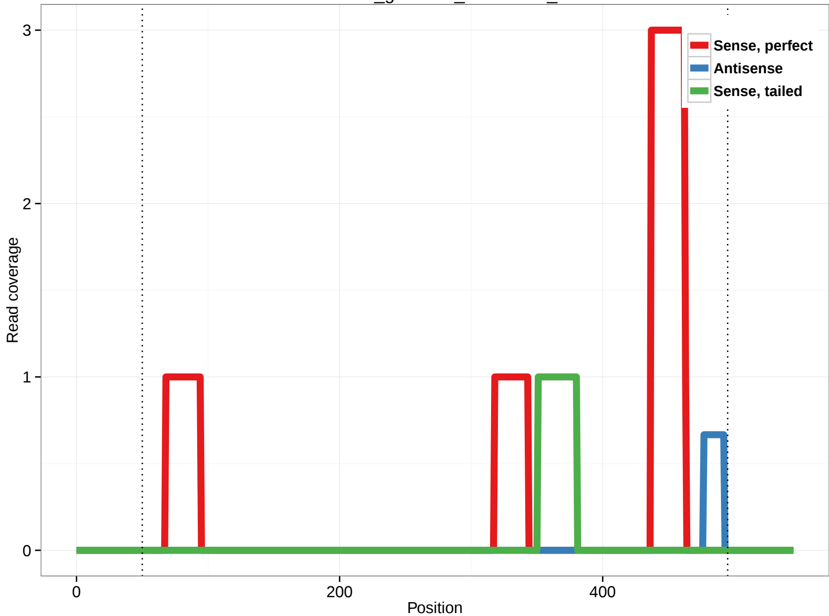
rheMac3_genscan_chr1.1373_2
