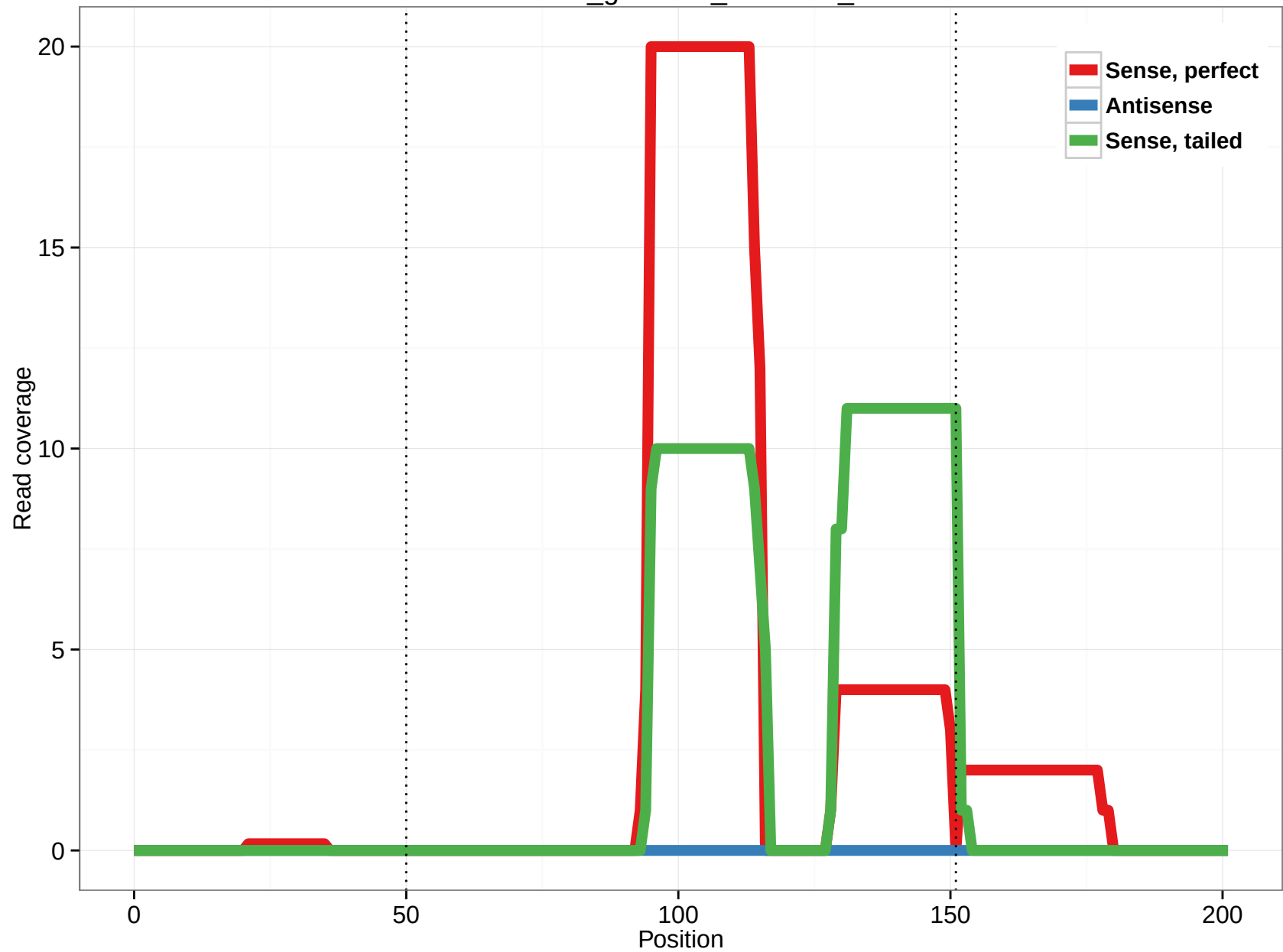
rheMac3_genscan_chr1.135_15
