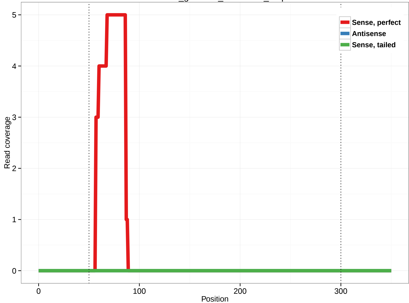
rheMac3_genscan_chr1.1349_4.3p
