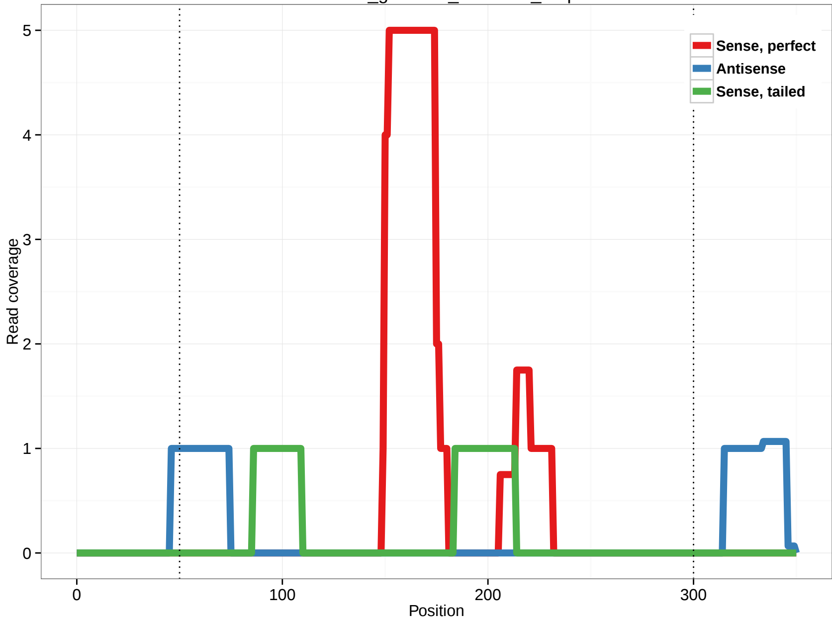
rheMac3_genscan_chr1.133_5.3p
