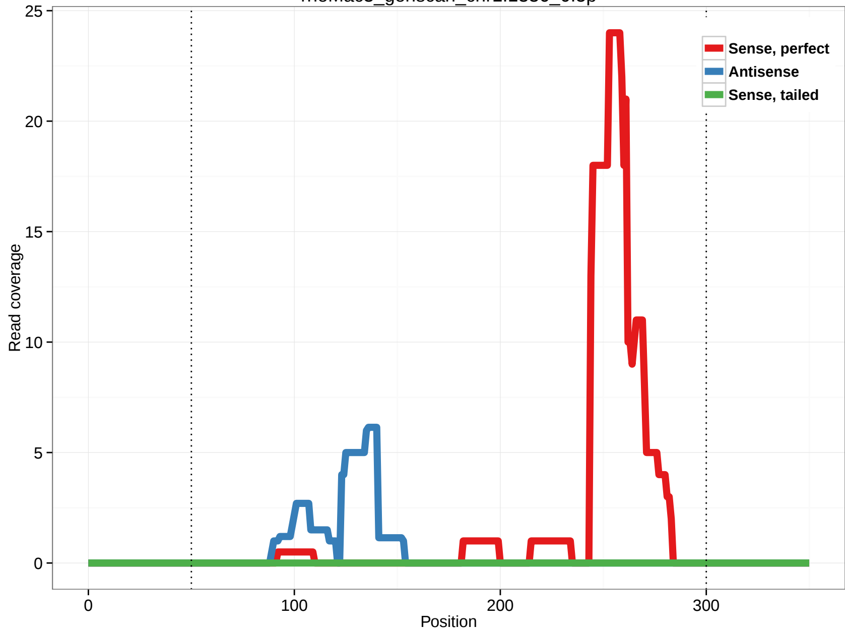
rheMac3_genscan_chr1.1336_0.5p
