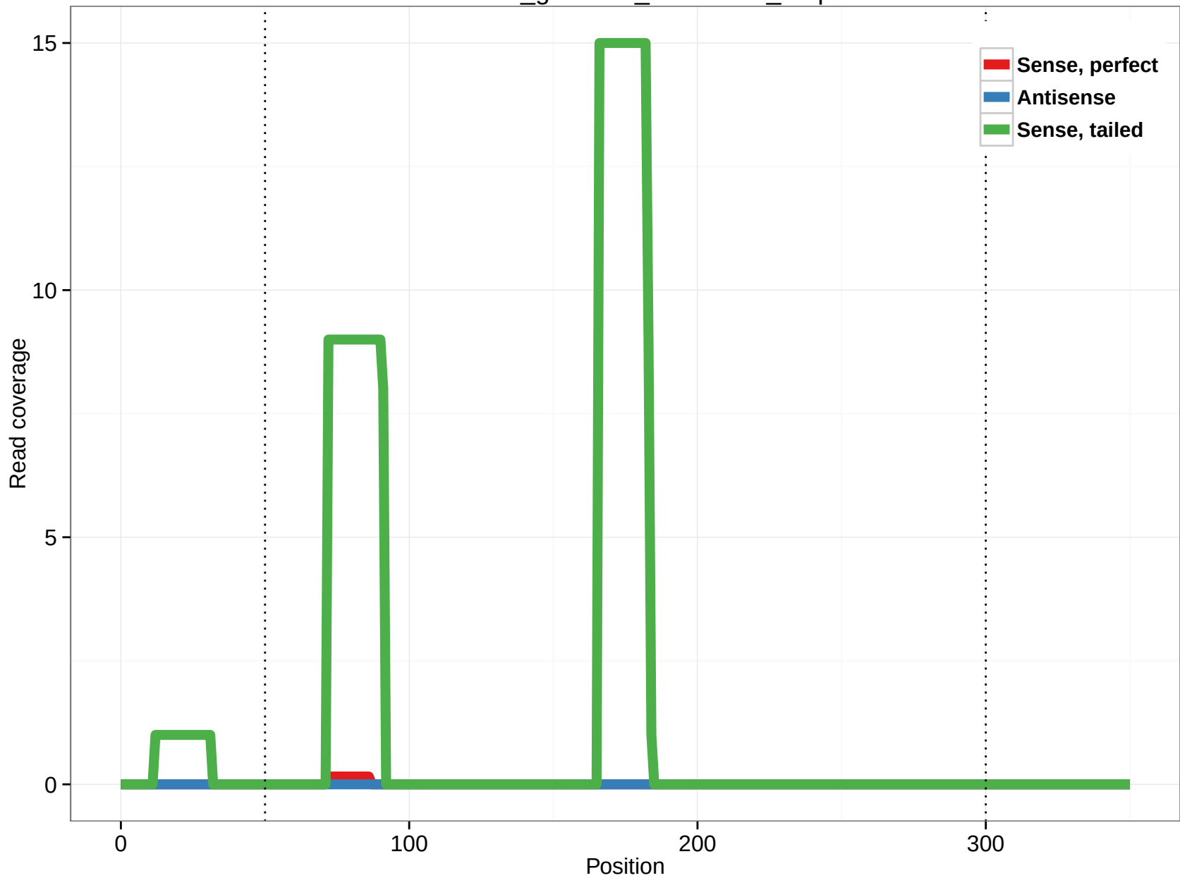
rheMac3_genscan_chr1.1263_5.5p
