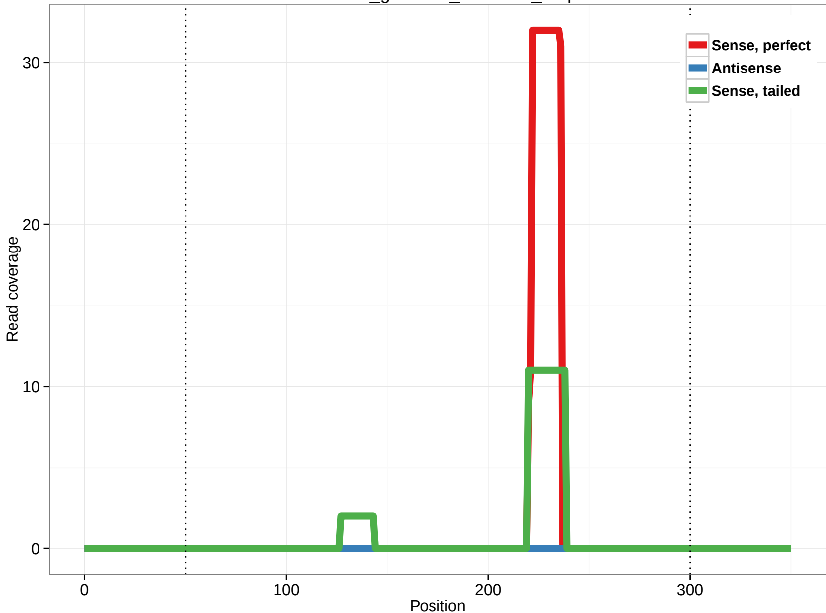
rheMac3_genscan_chr1.125_2.5p
