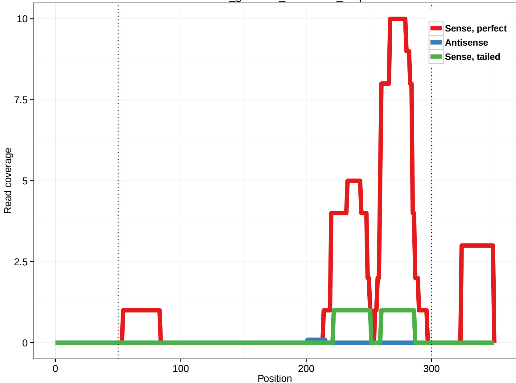
rheMac3_genscan_chr1.1240_8.5p
