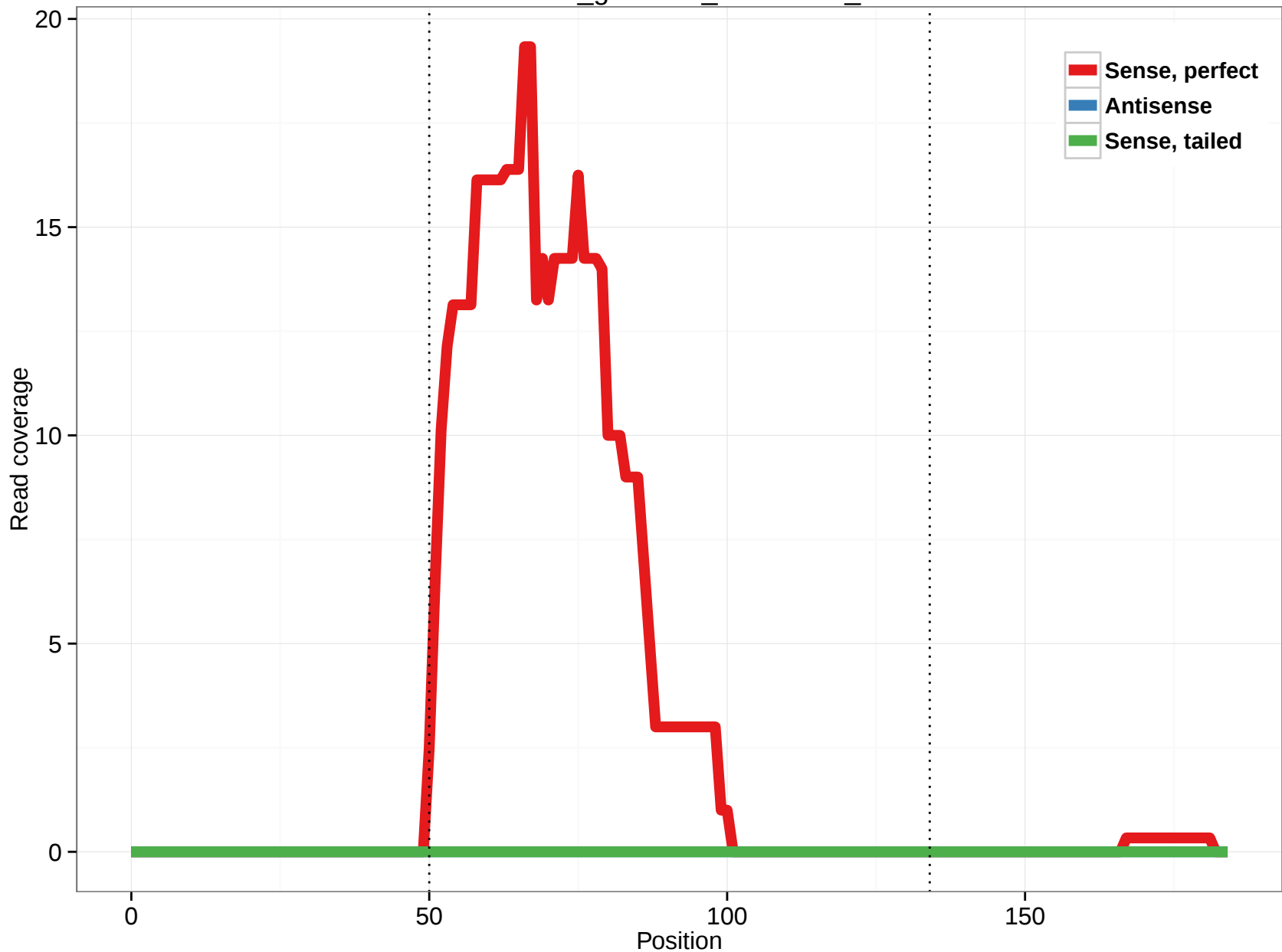
rheMac3_genscan_chr1.1199_15
