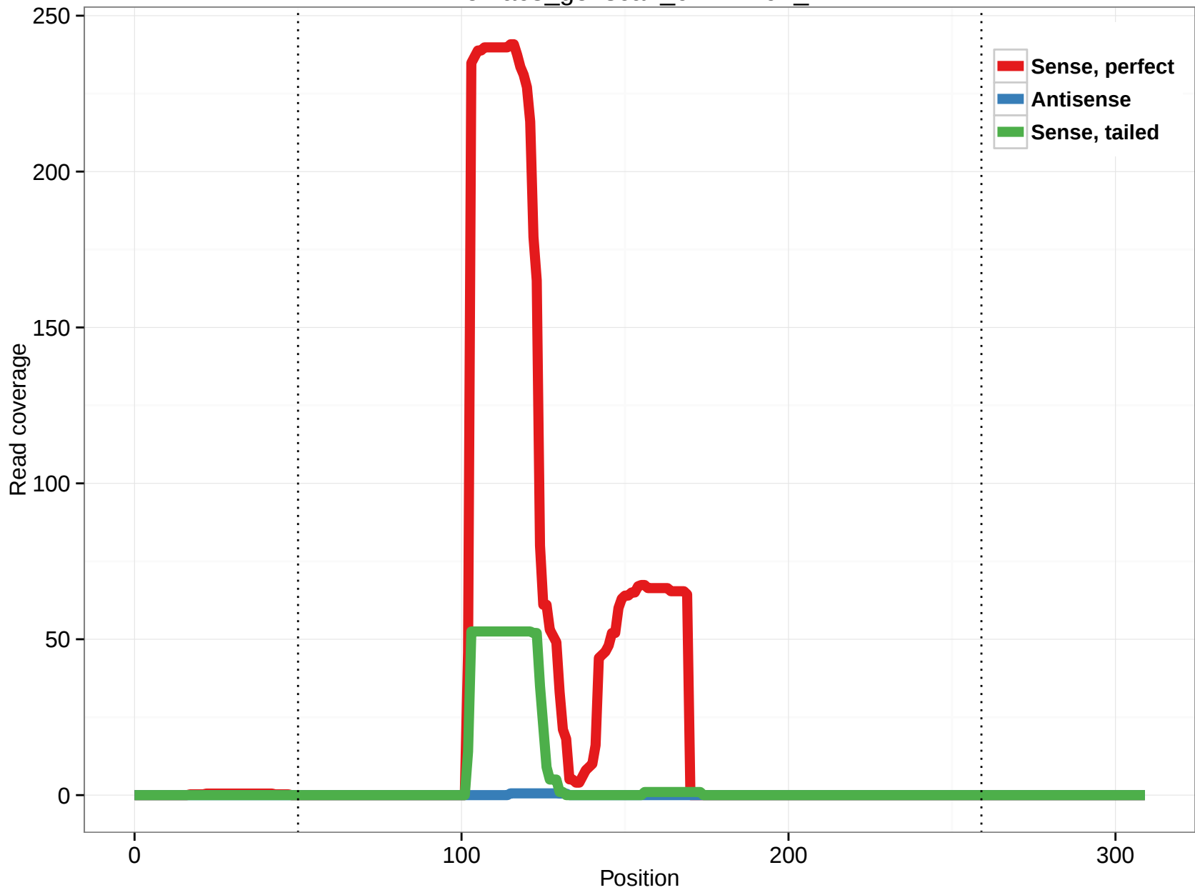
rheMac3_genscan_chr1.1194_22
