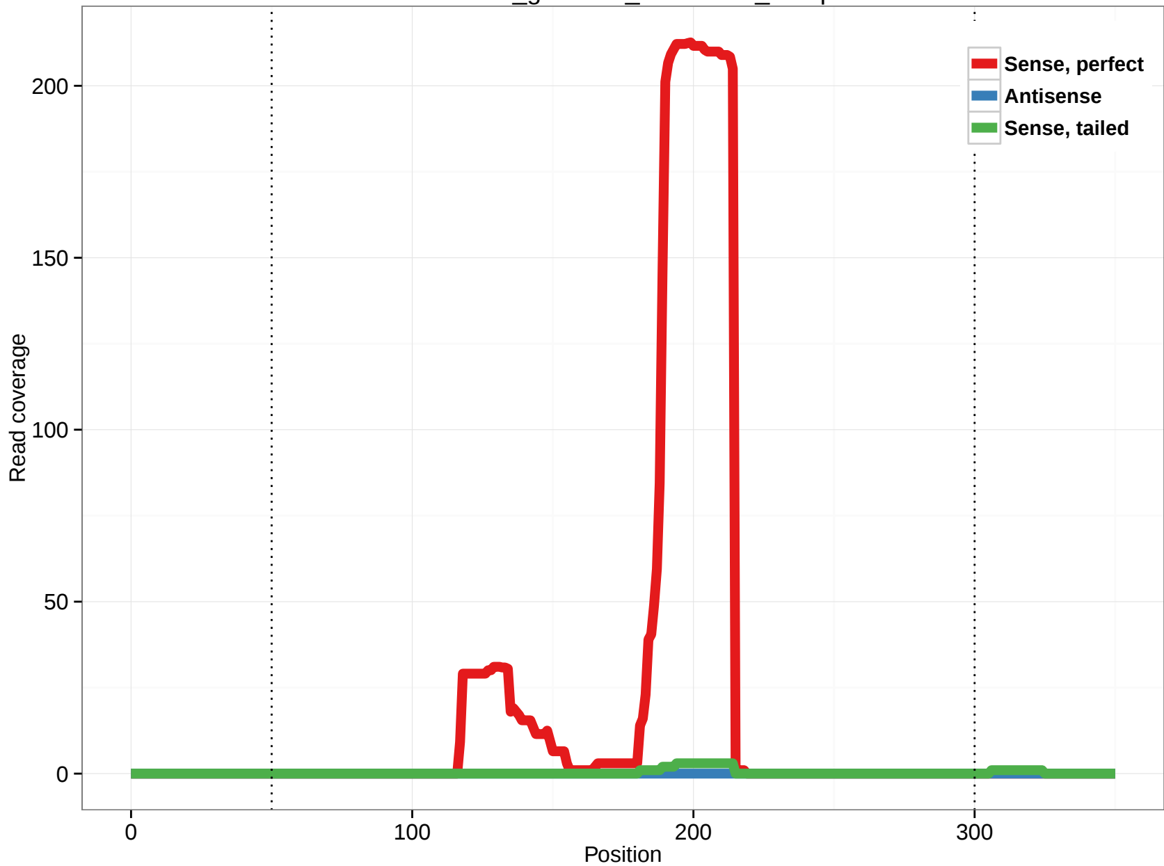
rheMac3_genscan_chr1.1194_20.3p
