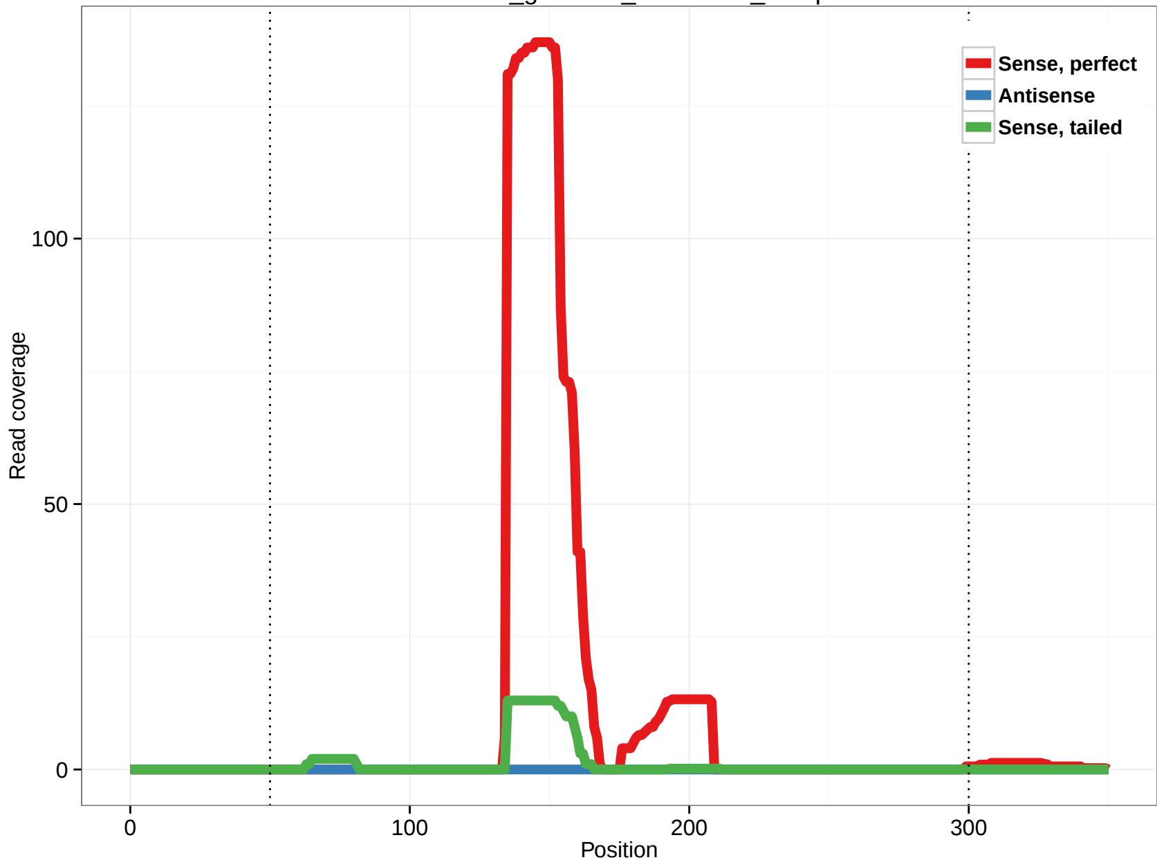
rheMac3_genscan_chr1.1194_19.3p
