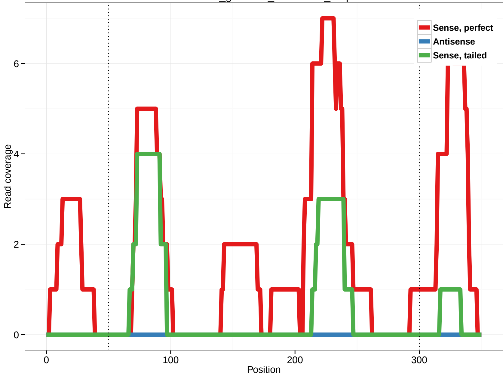
rheMac3_genscan_chr1.1107_5.5p
