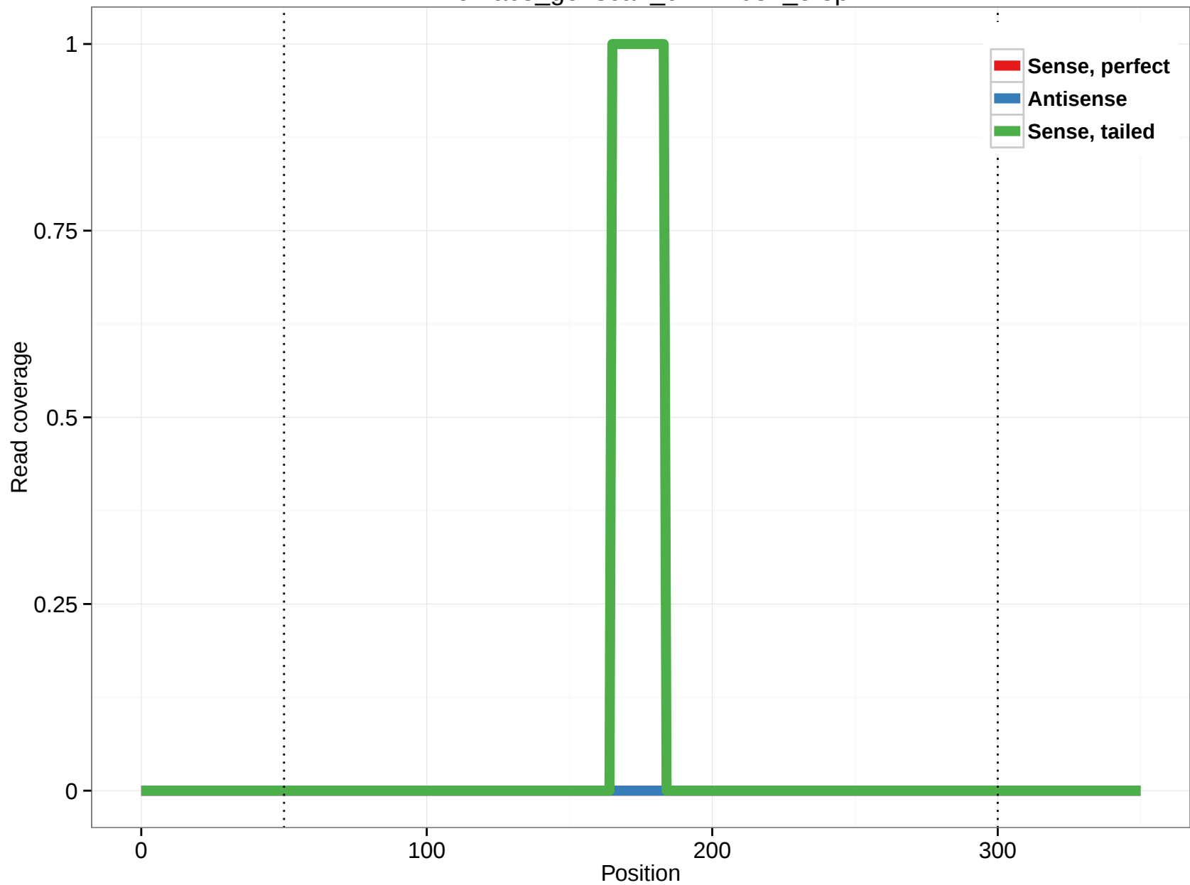
rheMac3_genscan_chr1.1087_5.3p
