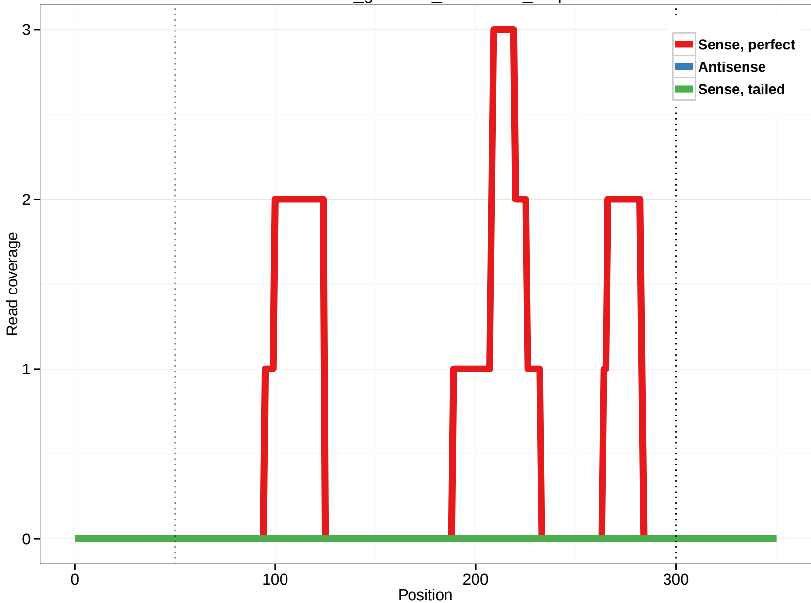
rheMac3_genscan_chr1.1055_9.5p
