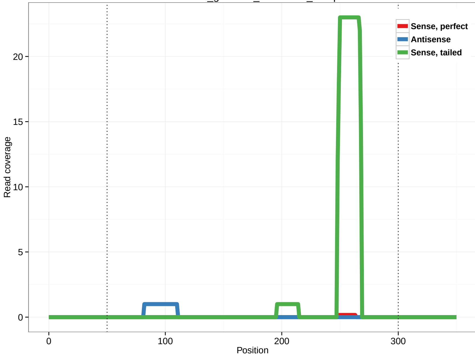
rheMac3_genscan_chr1.1003_28.5p
