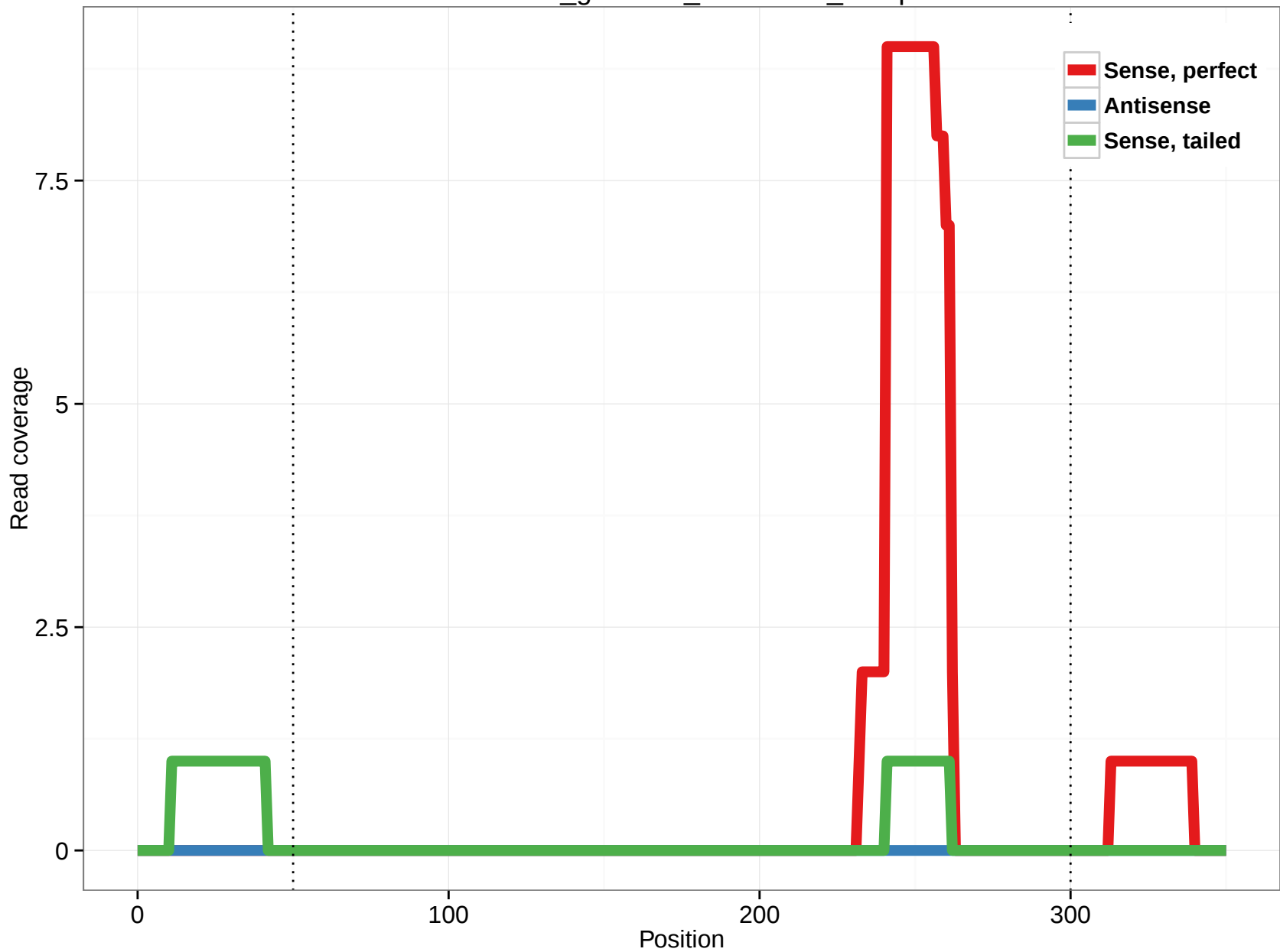
rheMac3_genscan_chr1.1003_19.3p
