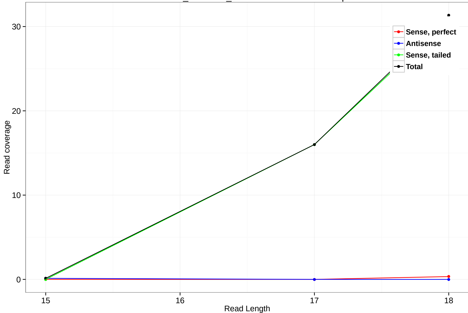
ornAna1_ensGene_ENSOANT00000023965.5p
