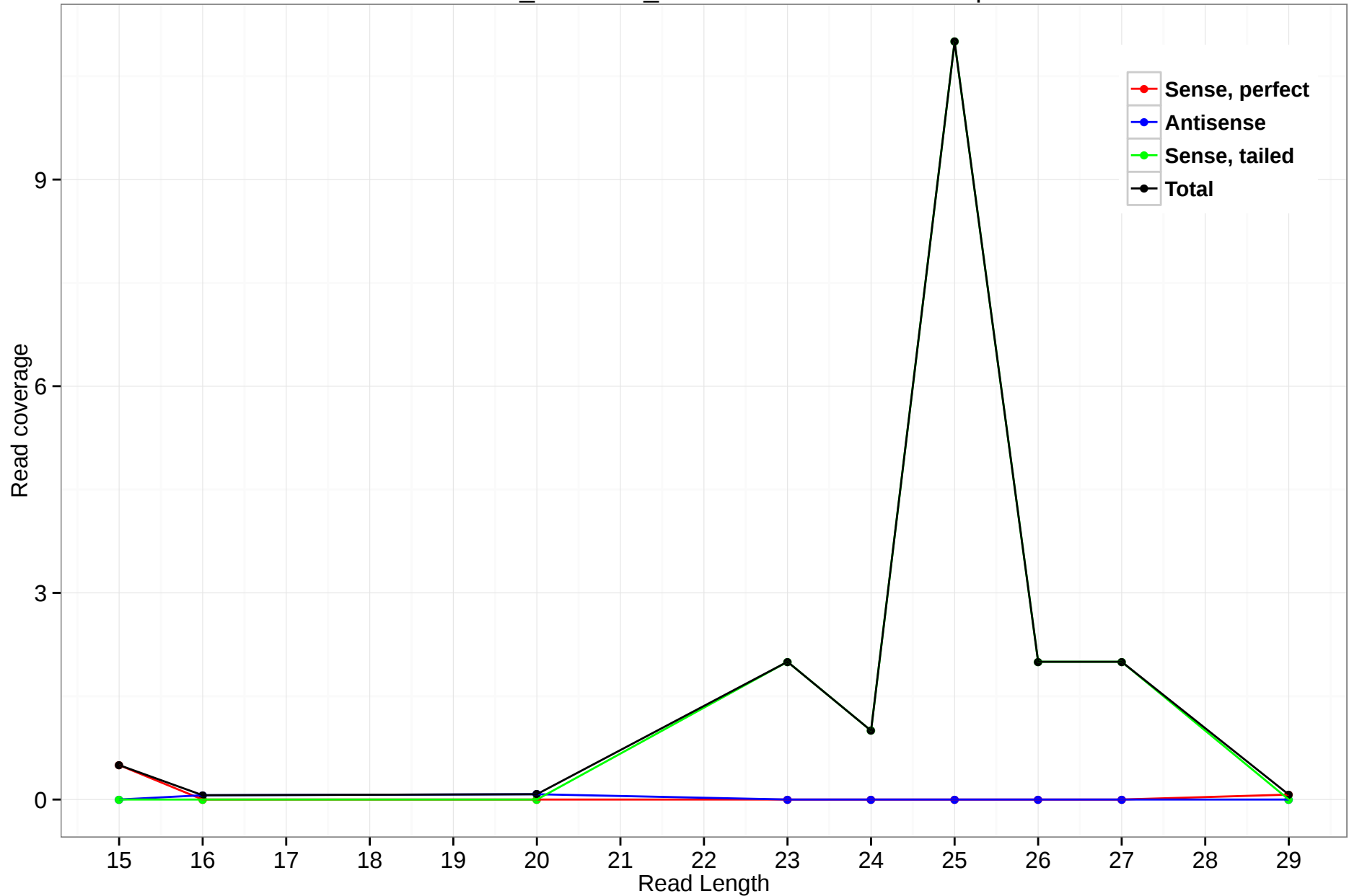
ornAna1_ensGene_ENSOANT00000022066.5p
