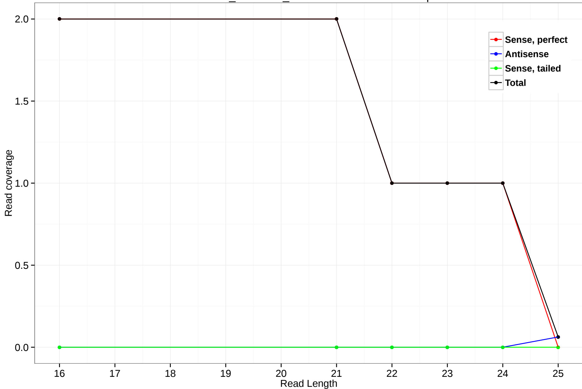
ornAna1_ensGene_ENSOANT00000021646.3p
