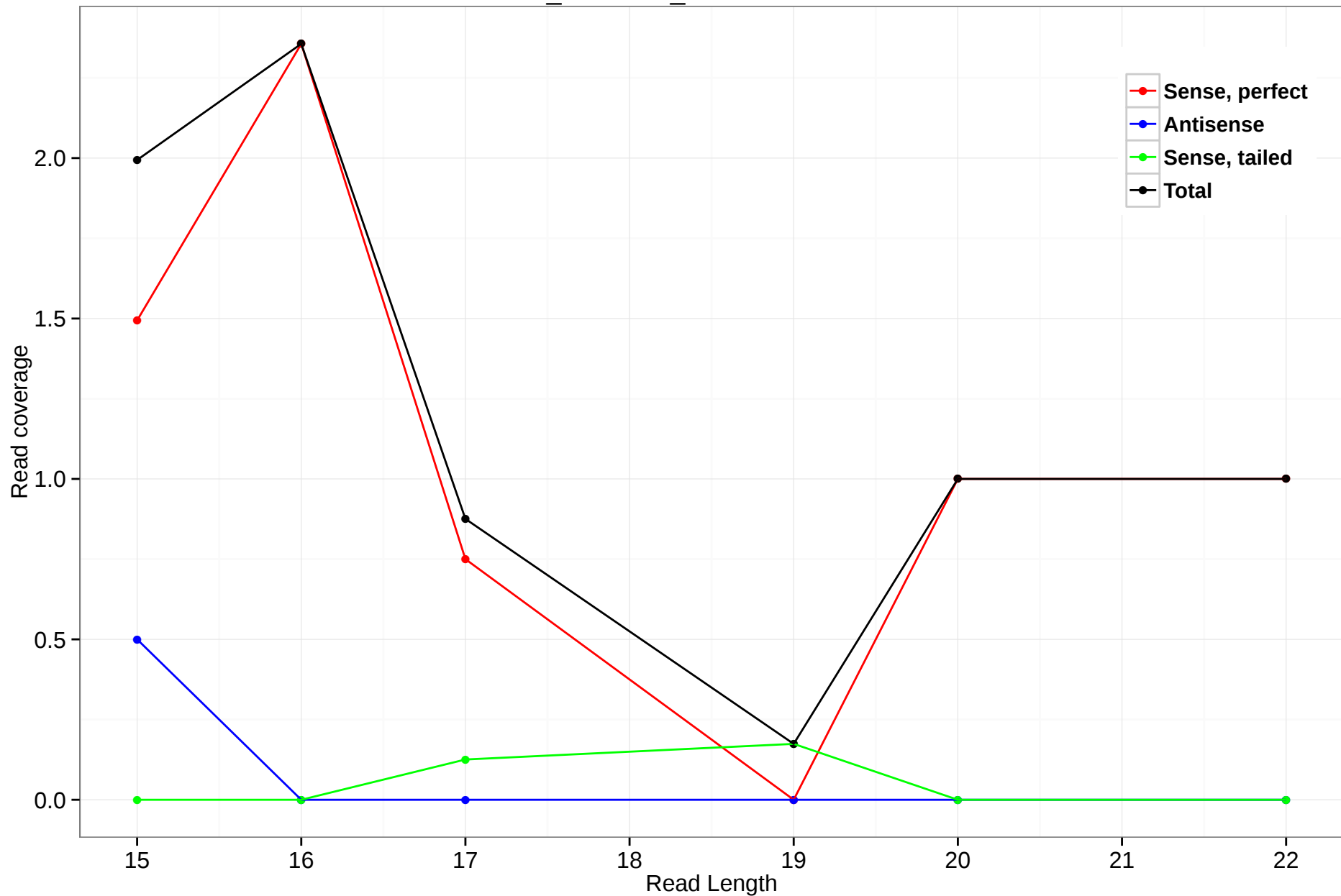
ornAna1_ensGene_ENSOANT00000017158
